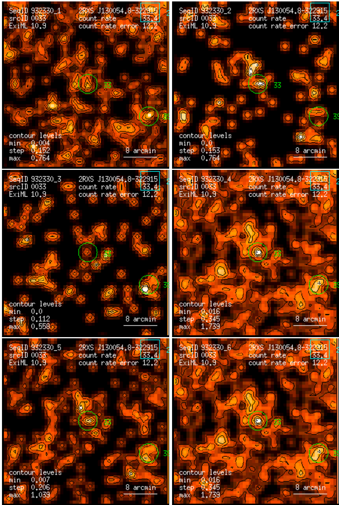
Figure 33: RASS 932330: detection 0033: band rate images, Gaussian filter: (1) PSPC channels 11 – 41, (2) 52 – 90, (3) 91 – 201, (4) 11 – 235, (5) 52 – 201, (6) 11 – 201. Broad band rates in counts/ks. Band rate contour levels in counts/ks/arcmin 2 .
