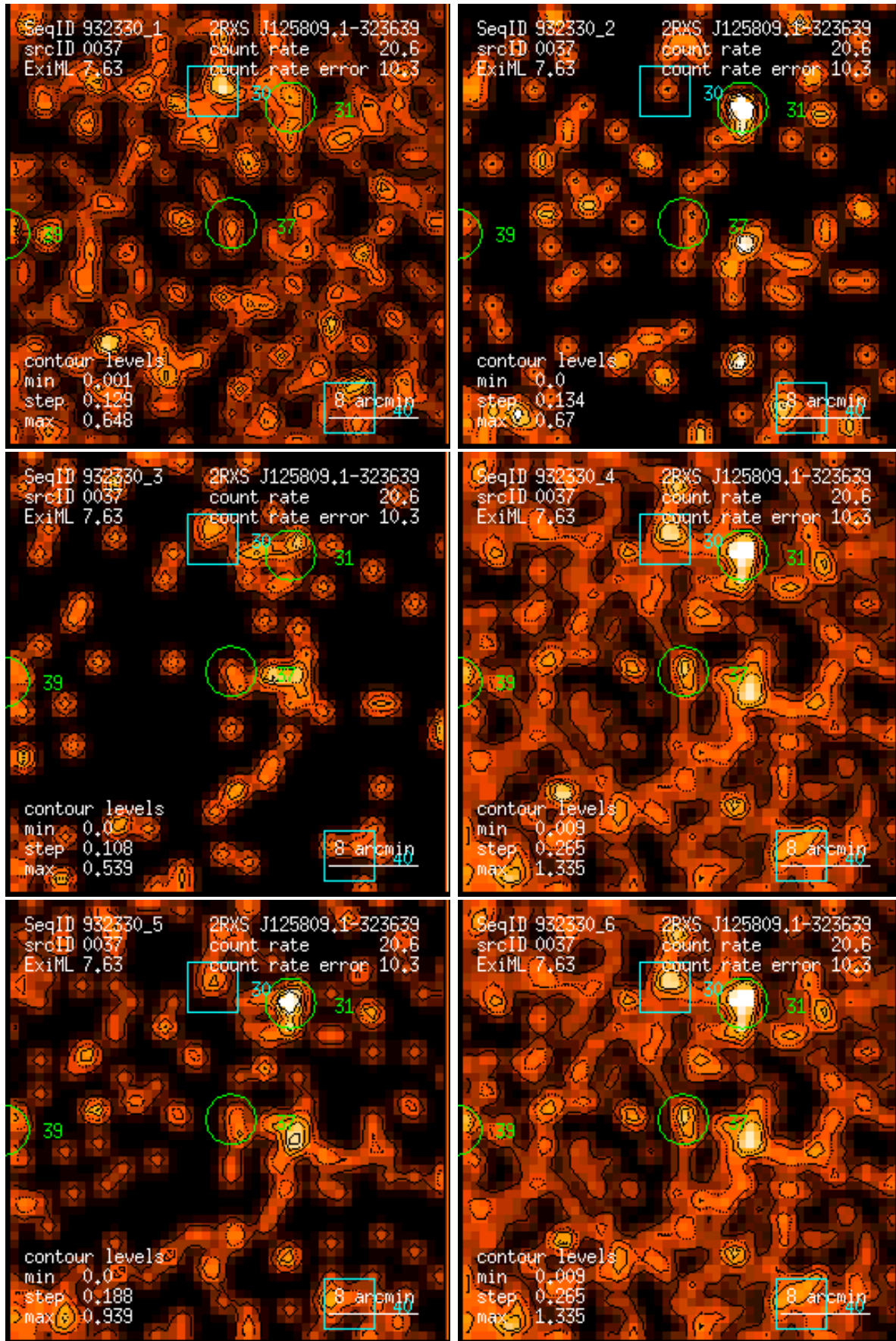
Figure 37: RASS 932330: detection 0037: band rate images, Gaussian filter: (1) PSPC channels 11 – 41, (2) 52 – 90, (3) 91 – 201, (4) 11 – 235, (5) 52 – 201, (6) 11 – 201. Broad band rates in counts/ks. Band rate contour levels in counts/ks/arcmin 2 .
