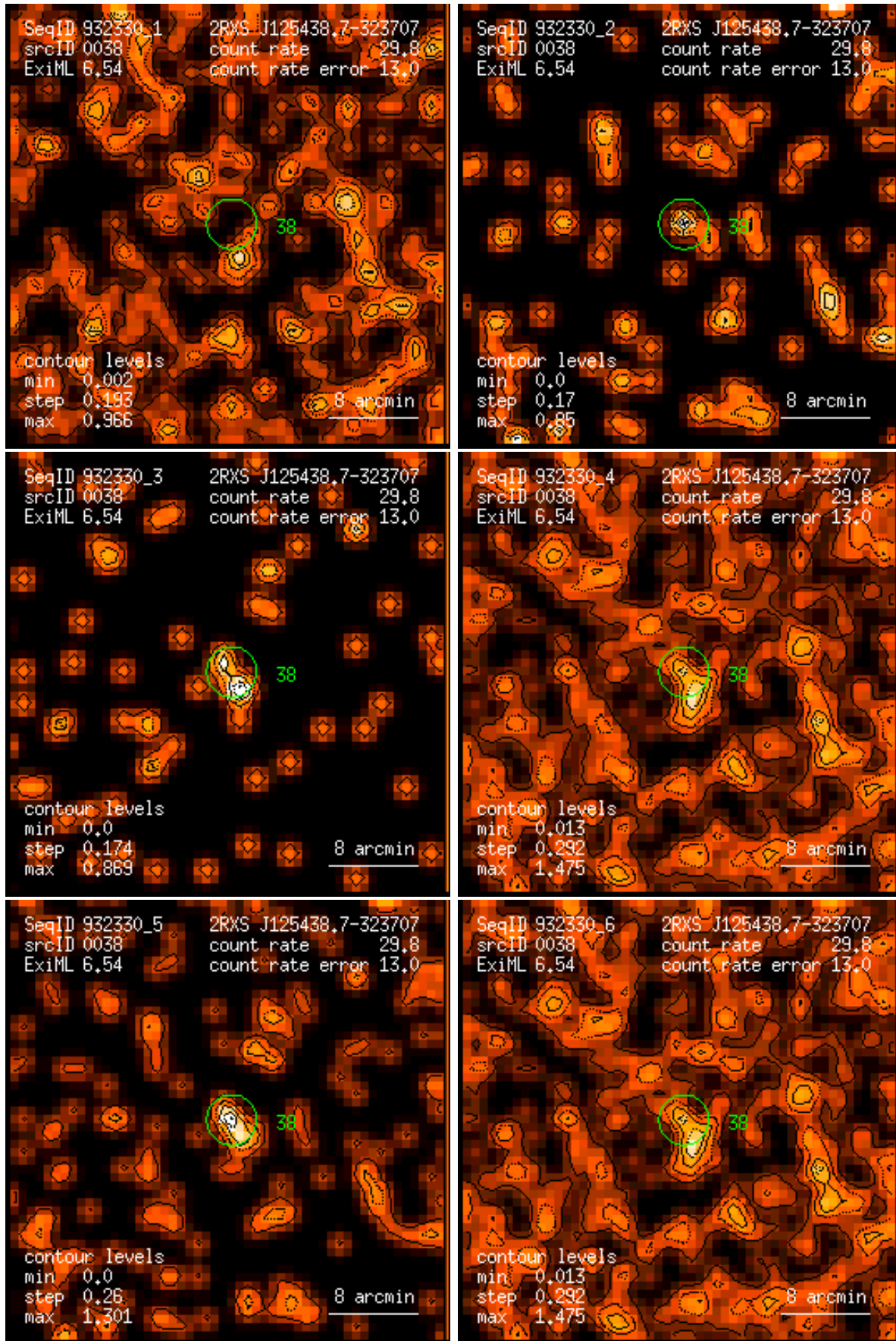
Figure 38: RASS 932330: detection 0038: band rate images, Gaussian filter: (1) PSPC channels 11 – 41, (2) 52 – 90, (3) 91 – 201, (4) 11 – 235, (5) 52 – 201, (6) 11 – 201. Broad band rates in counts/ks. Band rate contour levels in counts/ks/arcmin 2 .
