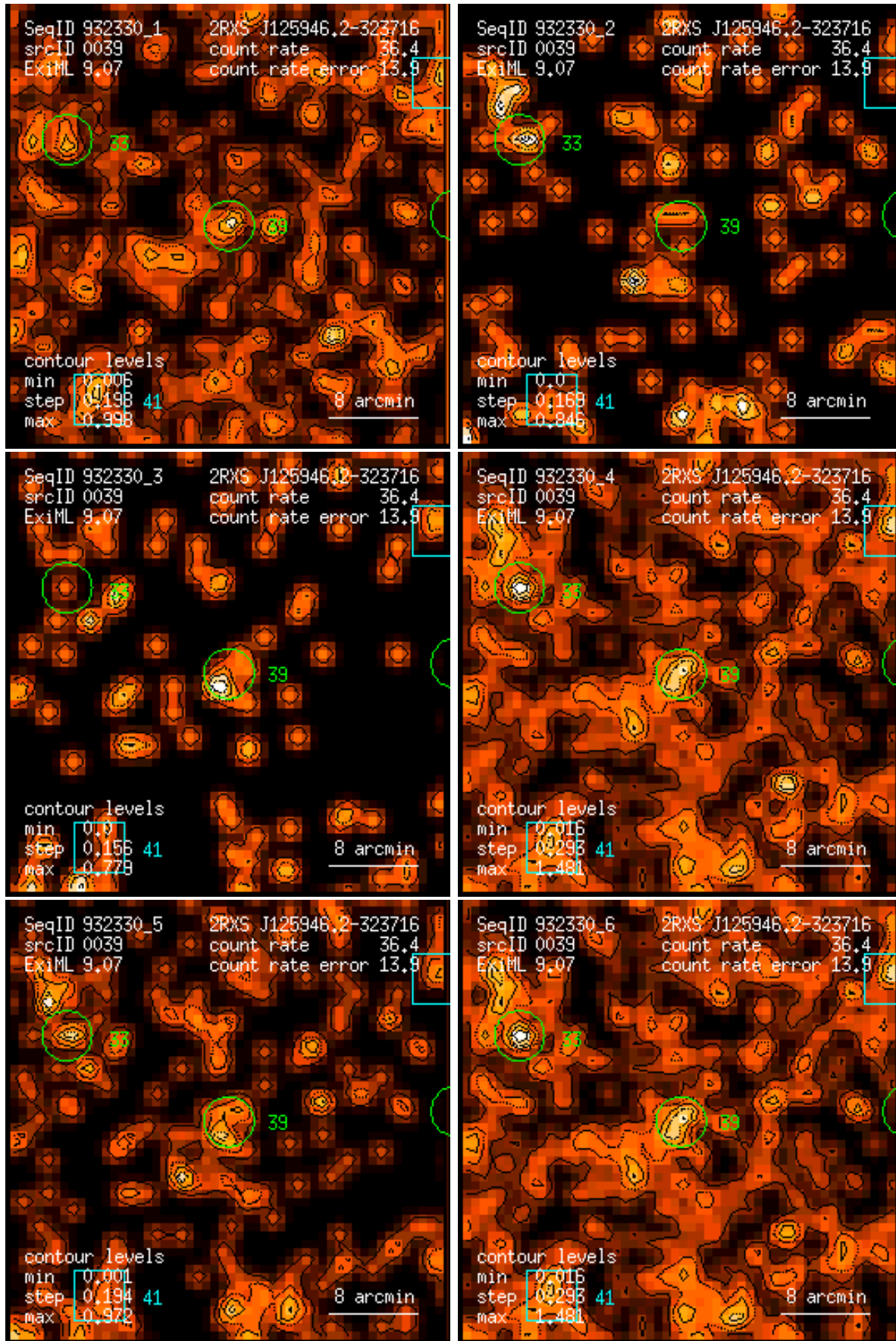
Figure 39: RASS 932330: detection 0039: band rate images, Gaussian filter: (1) PSPC channels 11 – 41, (2) 52 – 90, (3) 91 – 201, (4) 11 – 235, (5) 52 – 201, (6) 11 – 201. Broad band rates in counts/ks. Band rate contour levels in counts/ks/arcmin 2 .
