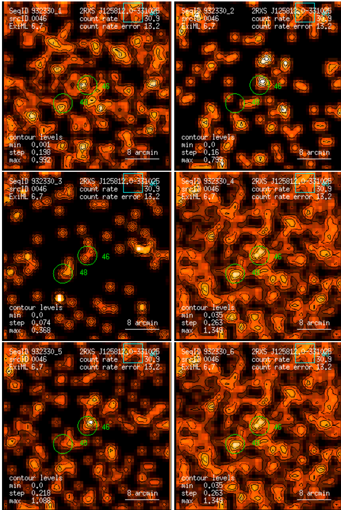
Figure 46: RASS 932330: detection 0046: band rate images, Gaussian filter: (1) PSPC channels 11 – 41, (2) 52 – 90, (3) 91 – 201, (4) 11 – 235, (5) 52 – 201, (6) 11 – 201. Broad band rates in counts/ks. Band rate contour levels in counts/ks/arcmin 2 .
