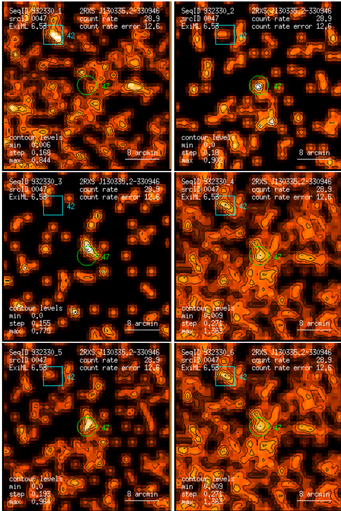
Figure 47: RASS 932330: detection 0047: band rate images, Gaussian filter: (1) PSPC channels 11 – 41, (2) 52 – 90, (3) 91 – 201, (4) 11 – 235, (5) 52 – 201, (6) 11 – 201. Broad band rates in counts/ks. Band rate contour levels in counts/ks/arcmin 2 .
