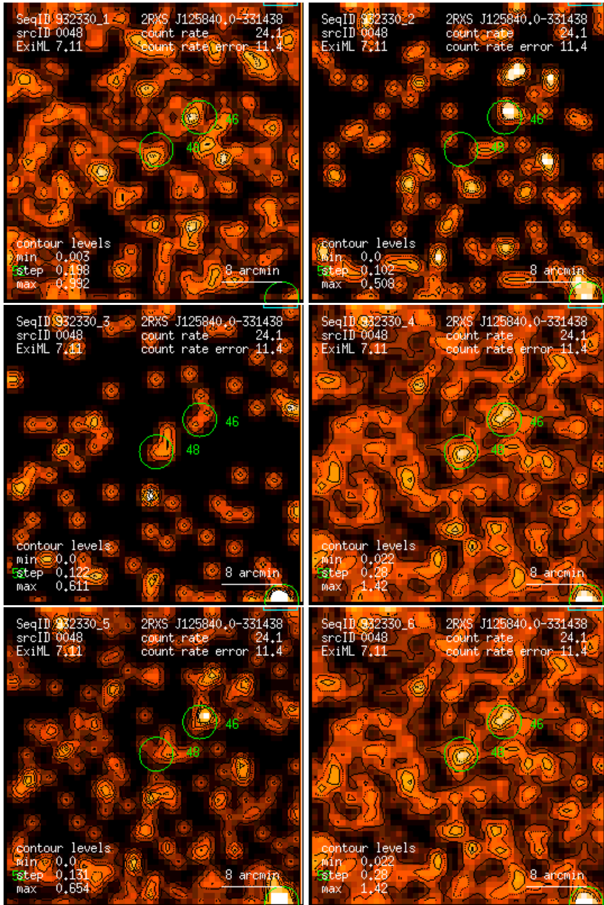
Figure 48: RASS 932330: detection 0048: band rate images, Gaussian filter: (1) PSPC channels 11 – 41, (2) 52 – 90, (3) 91 – 201, (4) 11 – 235, (5) 52 – 201, (6) 11 – 201. Broad band rates in counts/ks. Band rate contour levels in counts/ks/arcmin 2 .
