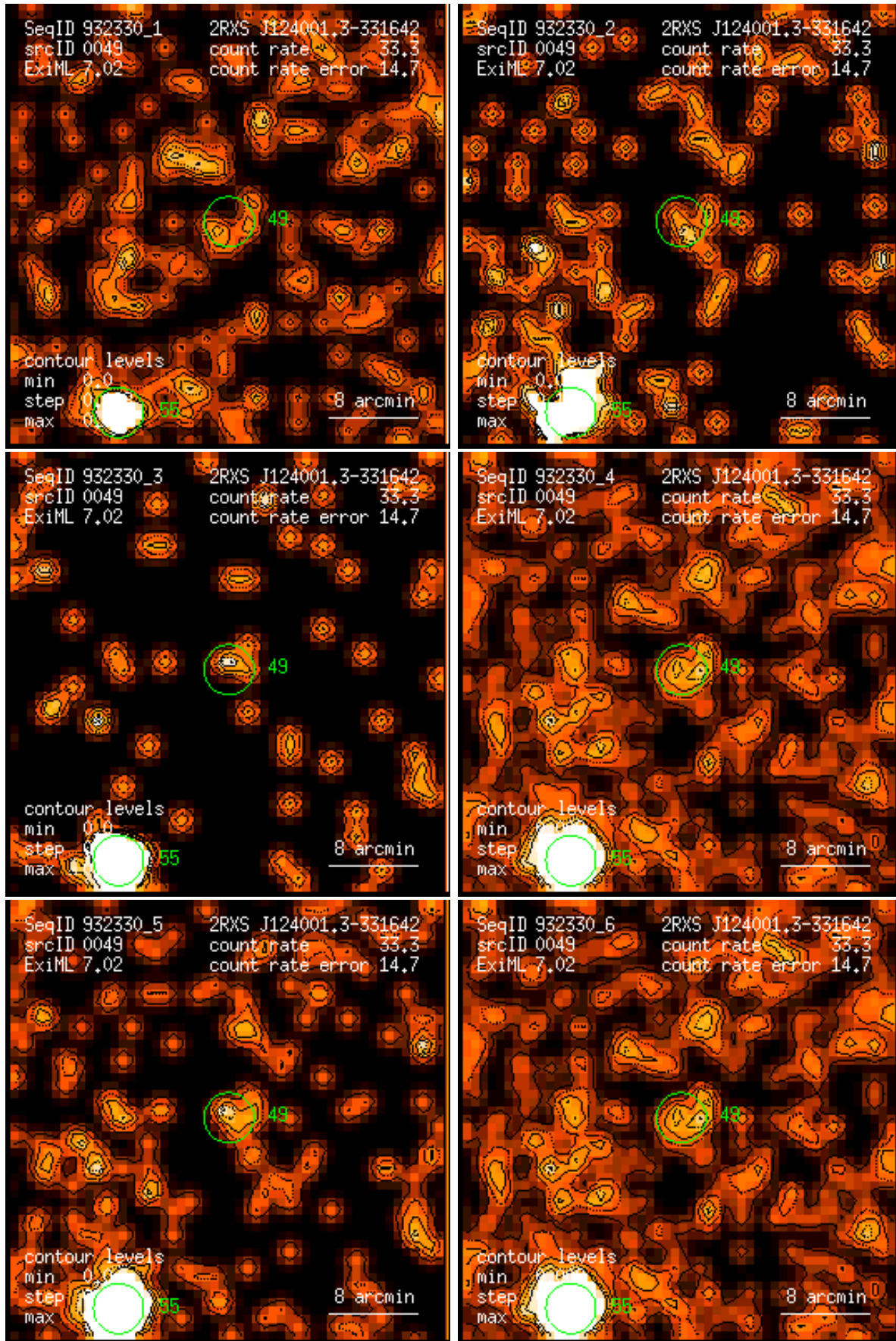
Figure 49: RASS 932330: detection 0049: band rate images, Gaussian filter: (1) PSPC channels 11 – 41, (2) 52 – 90, (3) 91 – 201, (4) 11 – 235, (5) 52 – 201, (6) 11 – 201. Broad band rates in counts/ks. Band rate contour levels in counts/ks/arcmin 2 .
