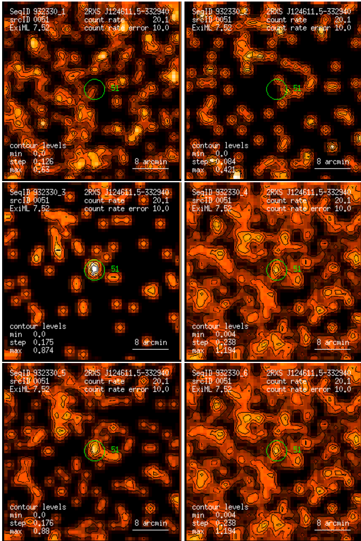
Figure 51: RASS 932330: detection 0051: band rate images, Gaussian filter: (1) PSPC channels 11 – 41, (2) 52 – 90, (3) 91 – 201, (4) 11 – 235, (5) 52 – 201, (6) 11 – 201. Broad band rates in counts/ks. Band rate contour levels in counts/ks/arcmin 2 .
