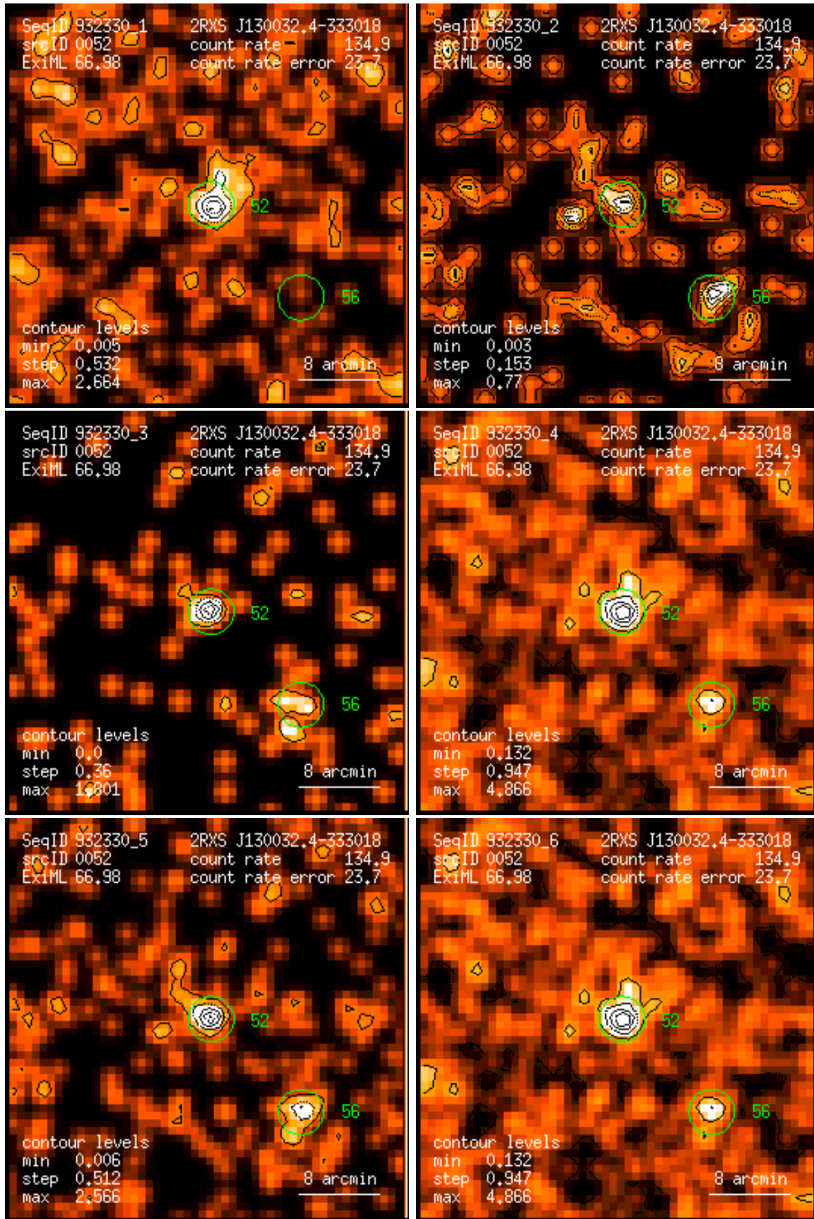
Figure 52: RASS 932330: detection 0052: band rate images, Gaussian filter: (1) PSPC channels 11 – 41, (2) 52 – 90, (3) 91 – 201, (4) 11 – 235, (5) 52 – 201, (6) 11 – 201. Broad band rates in counts/ks. Band rate contour levels in counts/ks/arcmin 2 .
