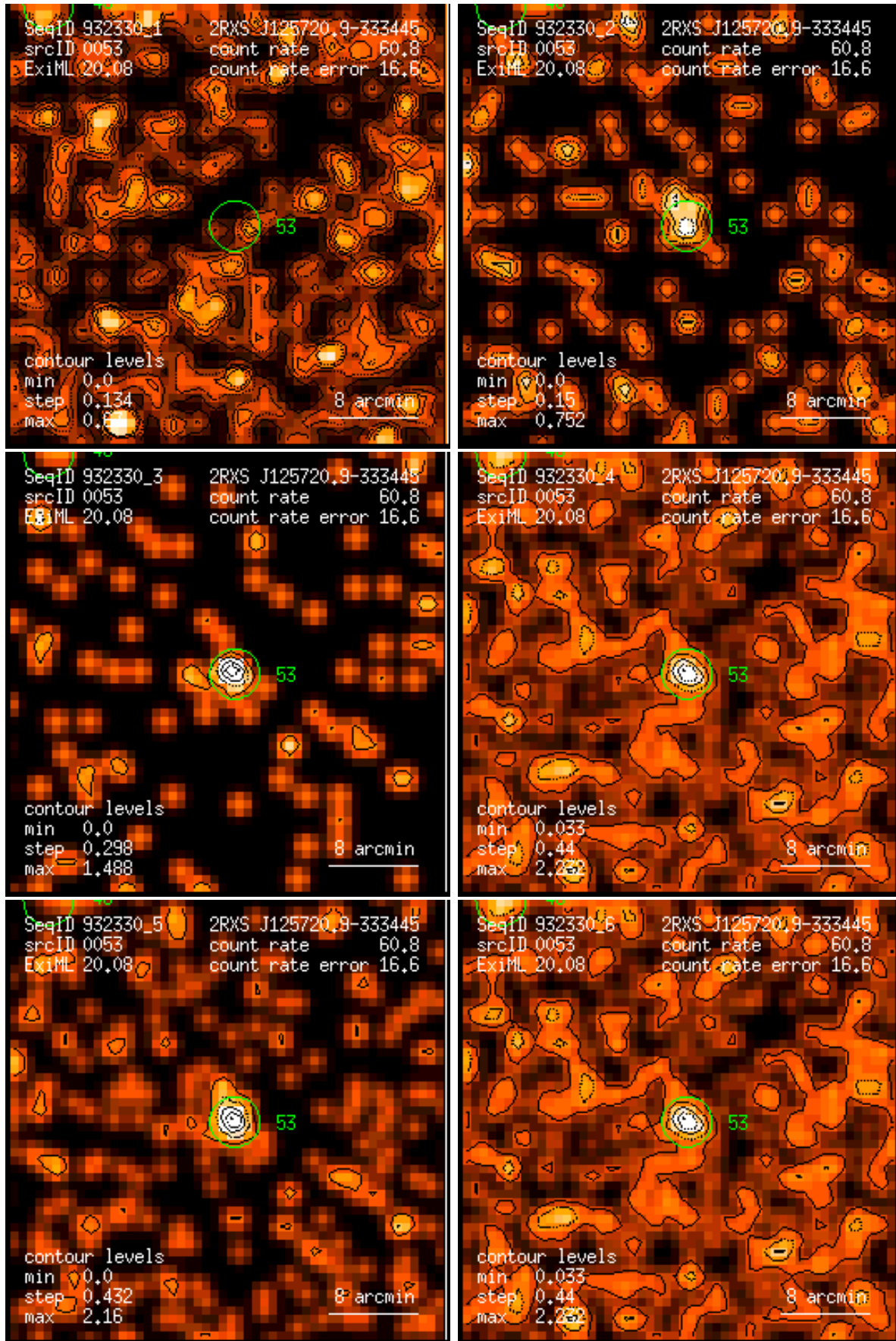
Figure 53: RASS 932330: detection 0053: band rate images, Gaussian filter: (1) PSPC channels 11 – 41, (2) 52 – 90, (3) 91 – 201, (4) 11 – 235, (5) 52 – 201, (6) 11 – 201. Broad band rates in counts/ks. Band rate contour levels in counts/ks/arcmin 2 .
