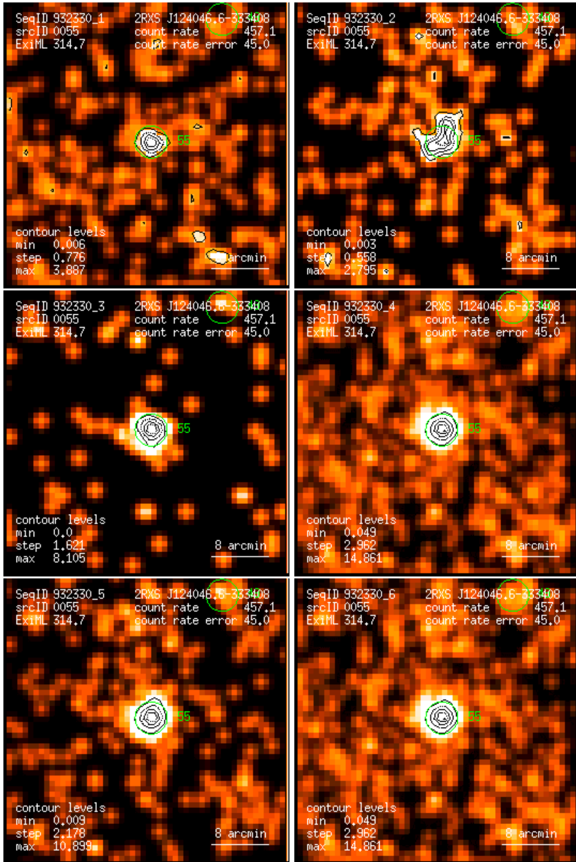
Figure 55: RASS 932330: detection 0055: band rate images, Gaussian filter: (1) PSPC channels 11 – 41, (2) 52 – 90, (3) 91 – 201, (4) 11 – 235, (5) 52 – 201, (6) 11 – 201. Broad band rates in counts/ks. Band rate contour levels in counts/ks/arcmin 2 .
