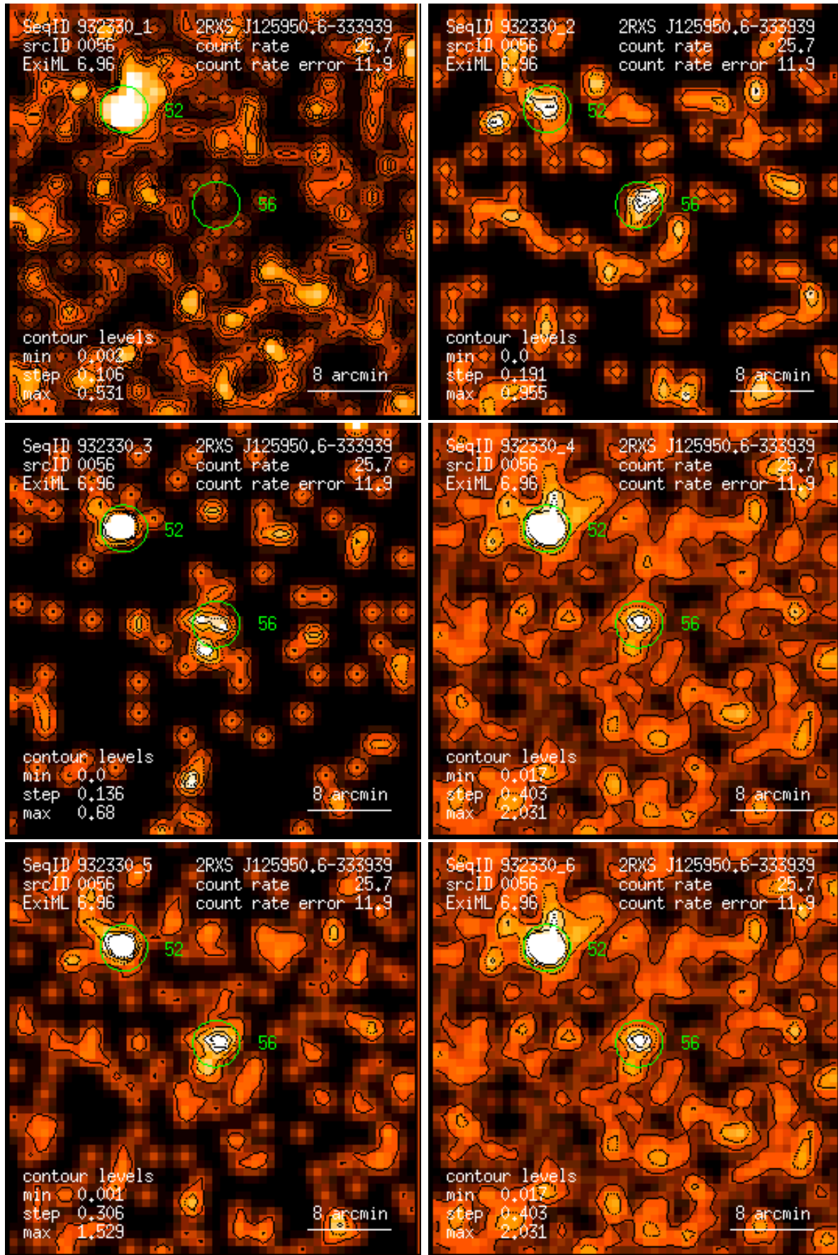
Figure 56: RASS 932330: detection 0056: band rate images, Gaussian filter: (1) PSPC channels 11 – 41, (2) 52 – 90, (3) 91 – 201, (4) 11 – 235, (5) 52 – 201, (6) 11 – 201. Broad band rates in counts/ks. Band rate contour levels in counts/ks/arcmin 2 .
