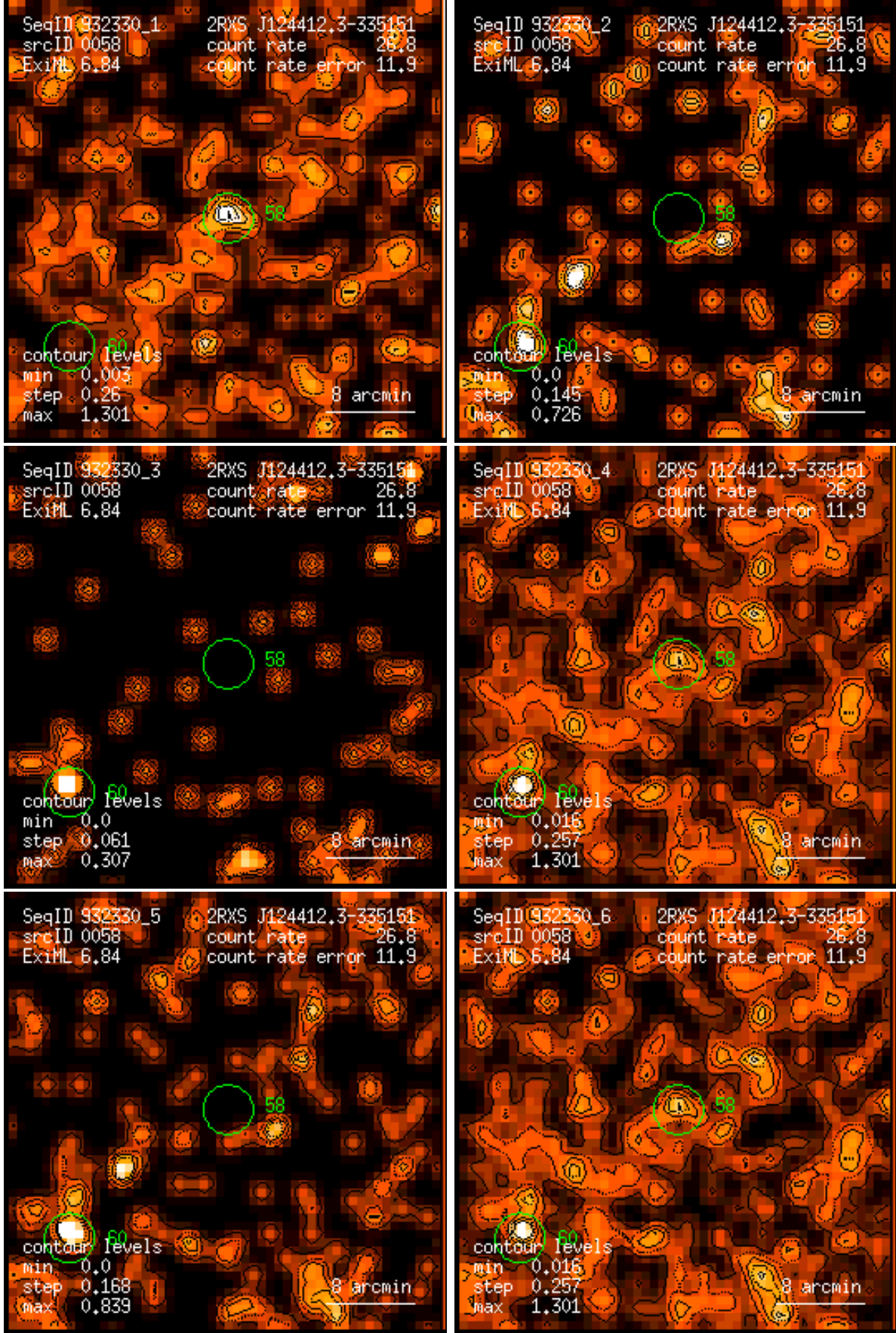
Figure 58: RASS 932330: detection 0058: band rate images, Gaussian filter: (1) PSPC channels 11 – 41, (2) 52 – 90, (3) 91 – 201, (4) 11 – 235, (5) 52 – 201, (6) 11 – 201. Broad band rates in counts/ks. Band rate contour levels in counts/ks/arcmin 2 .
