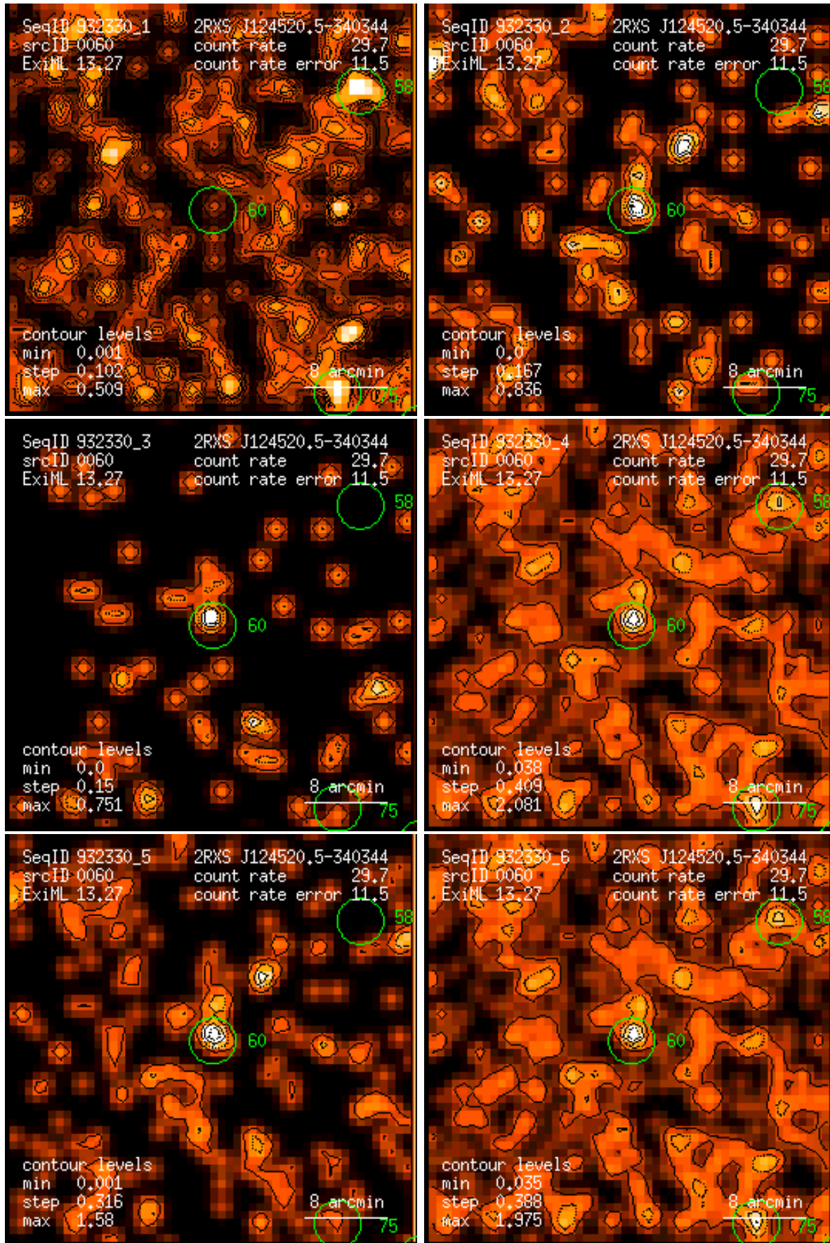
Figure 60: RASS 932330: detection 0060: band rate images, Gaussian filter: (1) PSPC channels 11 – 41, (2) 52 – 90, (3) 91 – 201, (4) 11 – 235, (5) 52 – 201, (6) 11 – 201. Broad band rates in counts/ks. Band rate contour levels in counts/ks/arcmin 2 .
