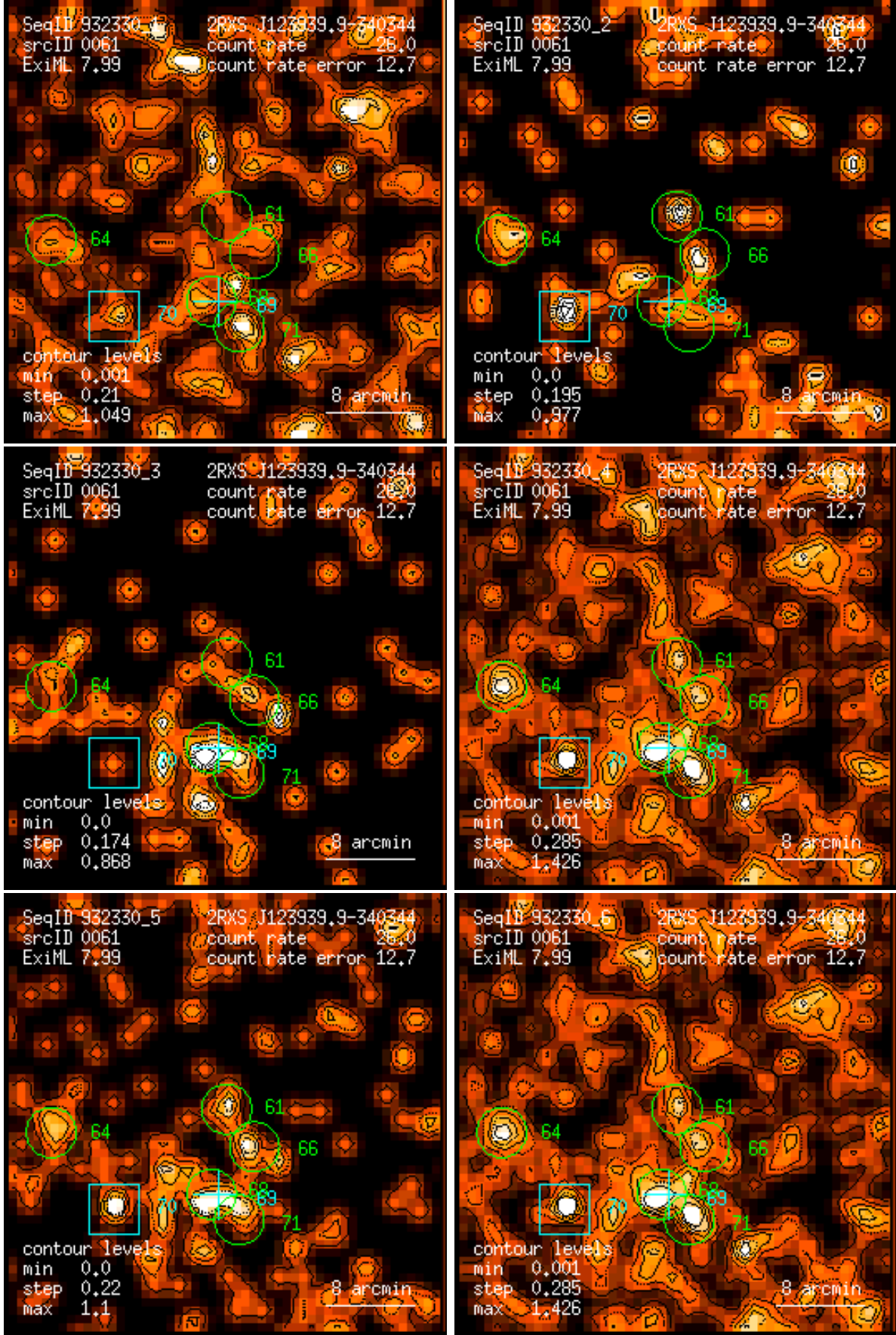
Figure 61: RASS 932330: detection 0061: band rate images, Gaussian filter: (1) PSPC channels 11 – 41, (2) 52 – 90, (3) 91 – 201, (4) 11 – 235, (5) 52 – 201, (6) 11 – 201. Broad band rates in counts/ks. Band rate contour levels in counts/ks/arcmin 2 .
