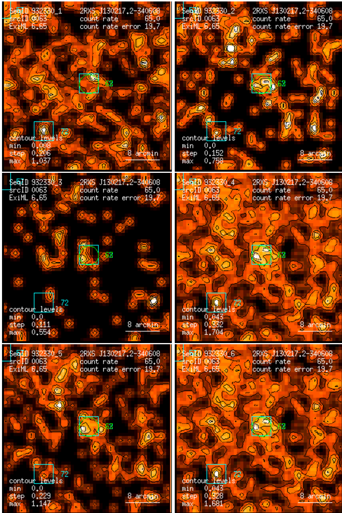
Figure 63: RASS 932330: detection 0063: band rate images, Gaussian filter: (1) PSPC channels 11 – 41, (2) 52 – 90, (3) 91 – 201, (4) 11 – 235, (5) 52 – 201, (6) 11 – 201. Broad band rates in counts/ks. Band rate contour levels in counts/ks/arcmin 2 .
