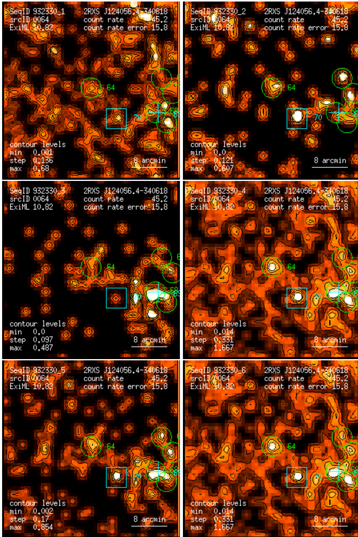
Figure 64: RASS 932330: detection 0064: band rate images, Gaussian filter: (1) PSPC channels 11 – 41, (2) 52 – 90, (3) 91 – 201, (4) 11 – 235, (5) 52 – 201, (6) 11 – 201. Broad band rates in counts/ks. Band rate contour levels in counts/ks/arcmin 2 .
