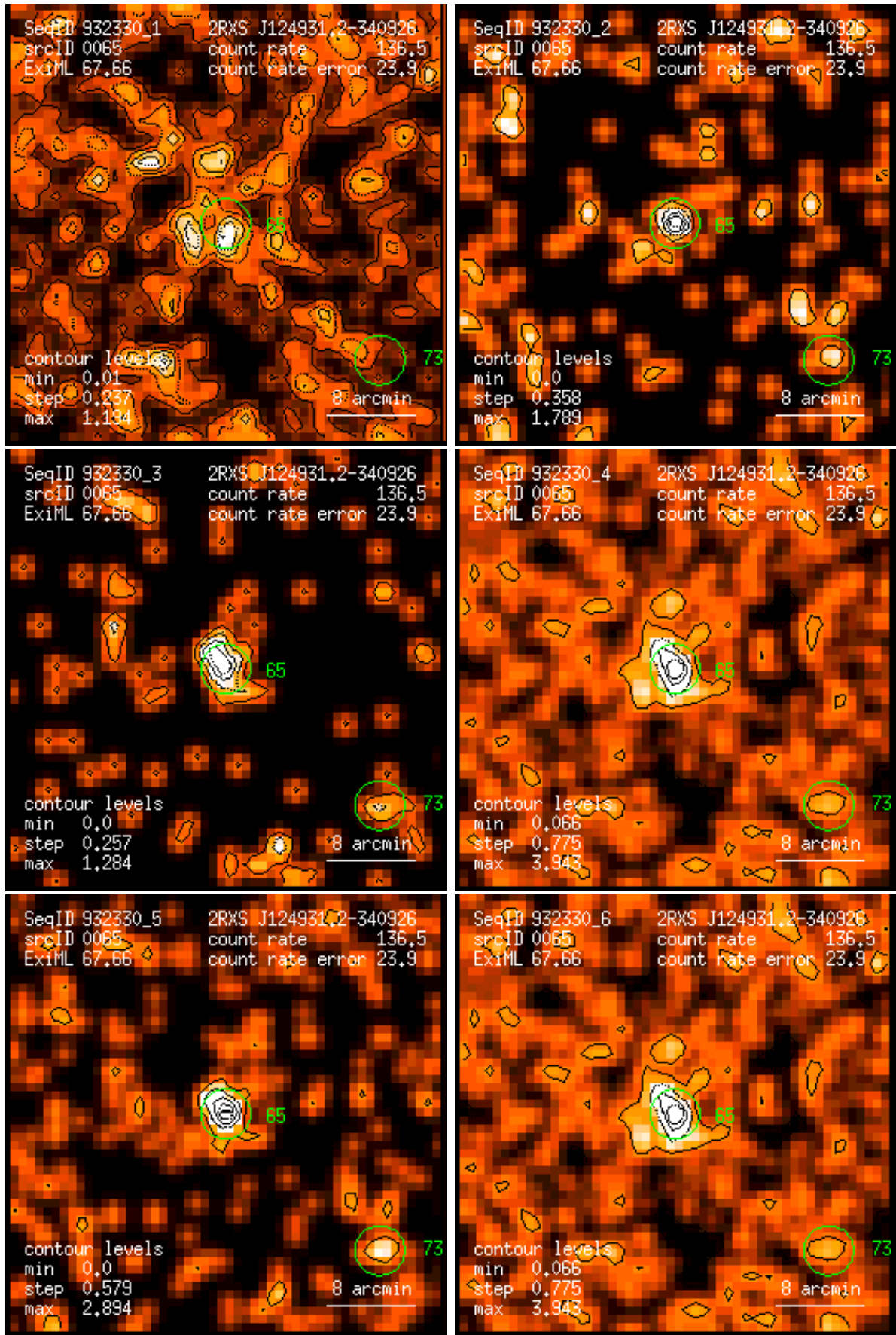
Figure 65: RASS 932330: detection 0065: band rate images, Gaussian filter: (1) PSPC channels 11 – 41, (2) 52 – 90, (3) 91 – 201, (4) 11 – 235, (5) 52 – 201, (6) 11 – 201. Broad band rates in counts/ks. Band rate contour levels in counts/ks/arcmin 2 .
