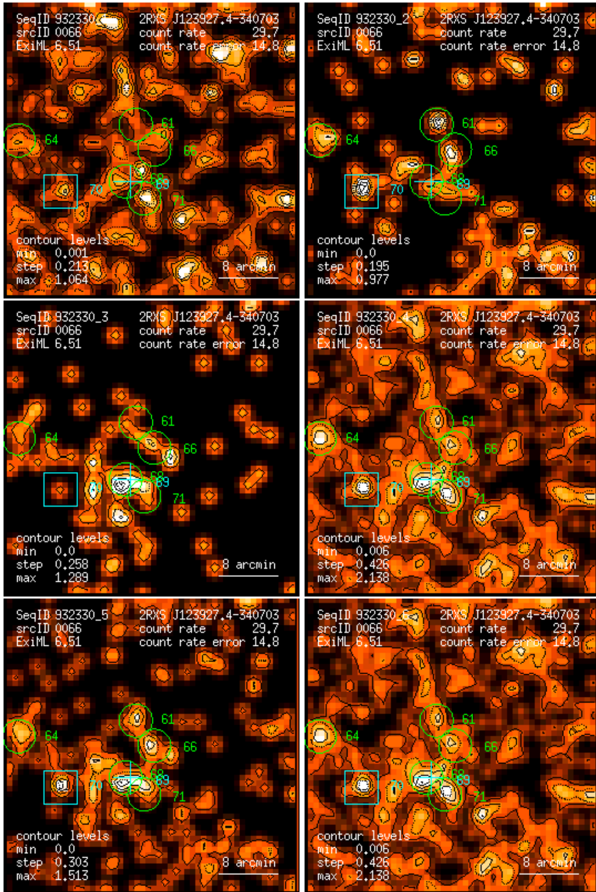
Figure 66: RASS 932330: detection 0066: band rate images, Gaussian filter: (1) PSPC channels 11 – 41, (2) 52 – 90, (3) 91 – 201, (4) 11 – 235, (5) 52 – 201, (6) 11 – 201. Broad band rates in counts/ks. Band rate contour levels in counts/ks/arcmin 2 .
