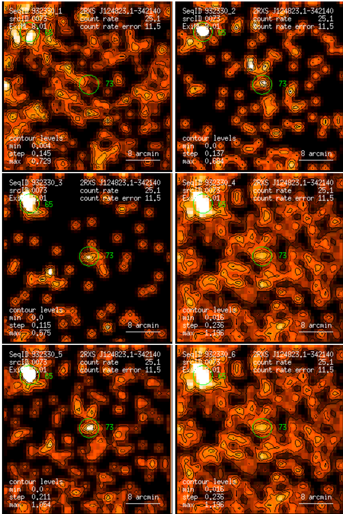
Figure 73: RASS 932330: detection 0073: band rate images, Gaussian filter: (1) PSPC channels 11 – 41, (2) 52 – 90, (3) 91 – 201, (4) 11 – 235, (5) 52 – 201, (6) 11 – 201. Broad band rates in counts/ks. Band rate contour levels in counts/ks/arcmin 2 .
