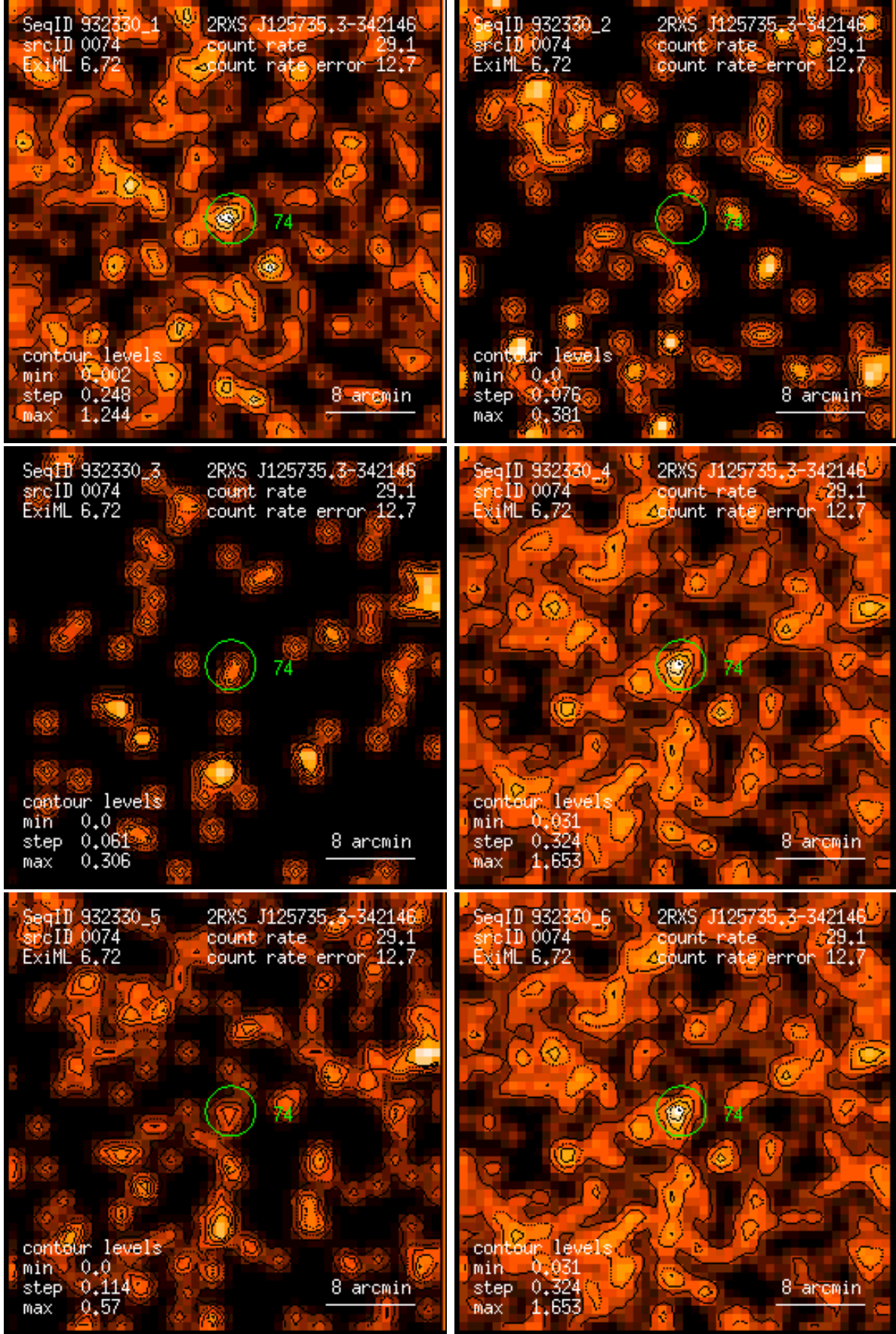
Figure 74: RASS 932330: detection 0074: band rate images, Gaussian filter: (1) PSPC channels 11 – 41, (2) 52 – 90, (3) 91 – 201, (4) 11 – 235, (5) 52 – 201, (6) 11 – 201. Broad band rates in counts/ks. Band rate contour levels in counts/ks/arcmin 2 .
