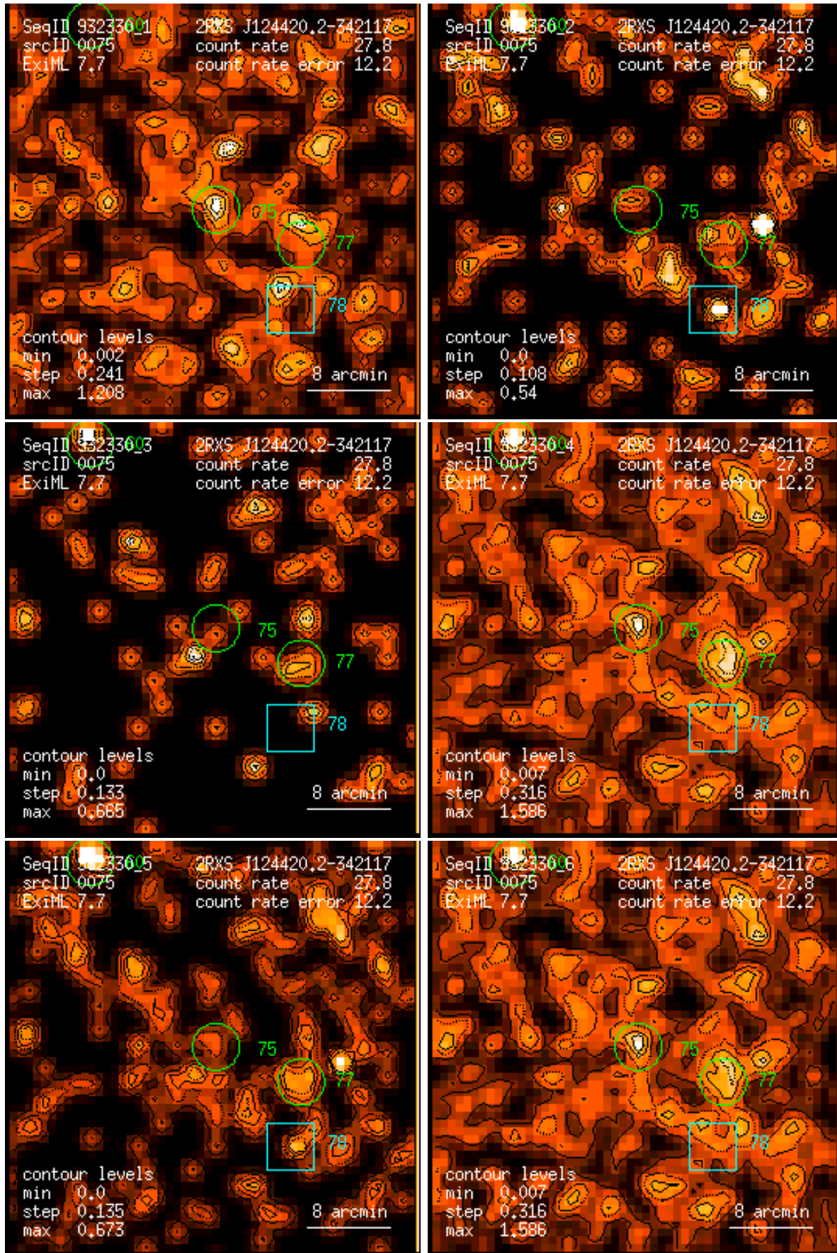
Figure 75: RASS 932330: detection 0075: band rate images, Gaussian filter: (1) PSPC channels 11 – 41, (2) 52 – 90, (3) 91 – 201, (4) 11 – 235, (5) 52 – 201, (6) 11 – 201. Broad band rates in counts/ks. Band rate contour levels in counts/ks/arcmin 2 .
