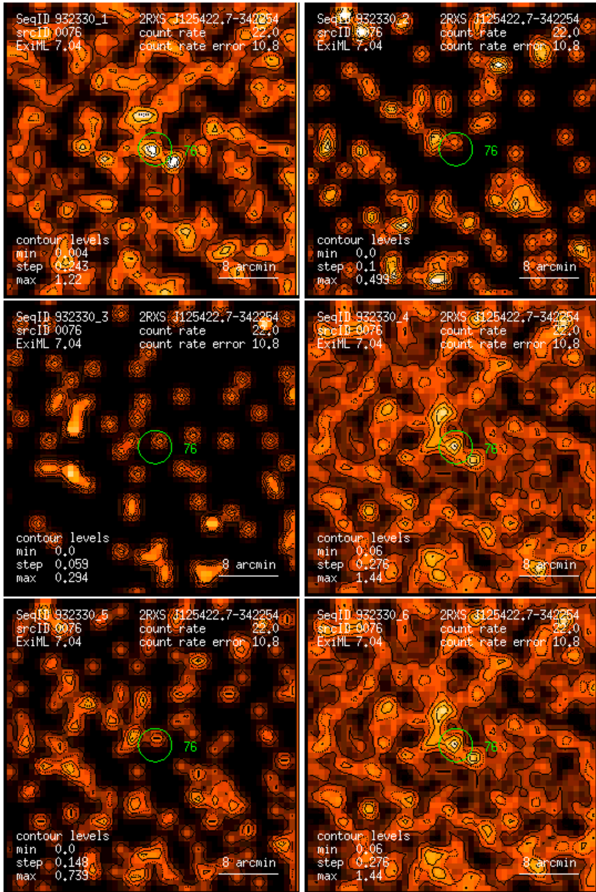
Figure 76: RASS 932330: detection 0076: band rate images, Gaussian filter: (1) PSPC channels 11 – 41, (2) 52 – 90, (3) 91 – 201, (4) 11 – 235, (5) 52 – 201, (6) 11 – 201. Broad band rates in counts/ks. Band rate contour levels in counts/ks/arcmin 2 .
