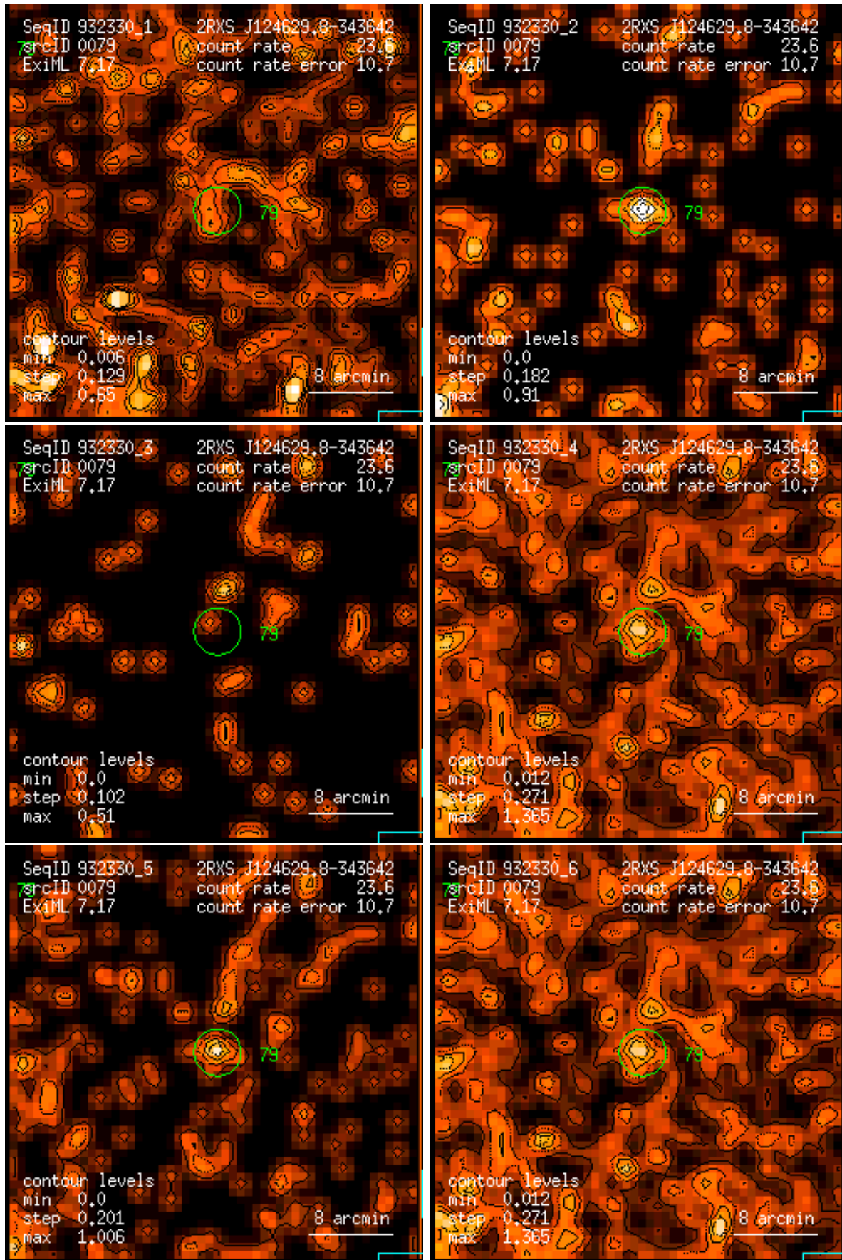
Figure 79: RASS 932330: detection 0079: band rate images, Gaussian filter: (1) PSPC channels 11 – 41, (2) 52 – 90, (3) 91 – 201, (4) 11 – 235, (5) 52 – 201, (6) 11 – 201. Broad band rates in counts/ks. Band rate contour levels in counts/ks/arcmin 2 .
