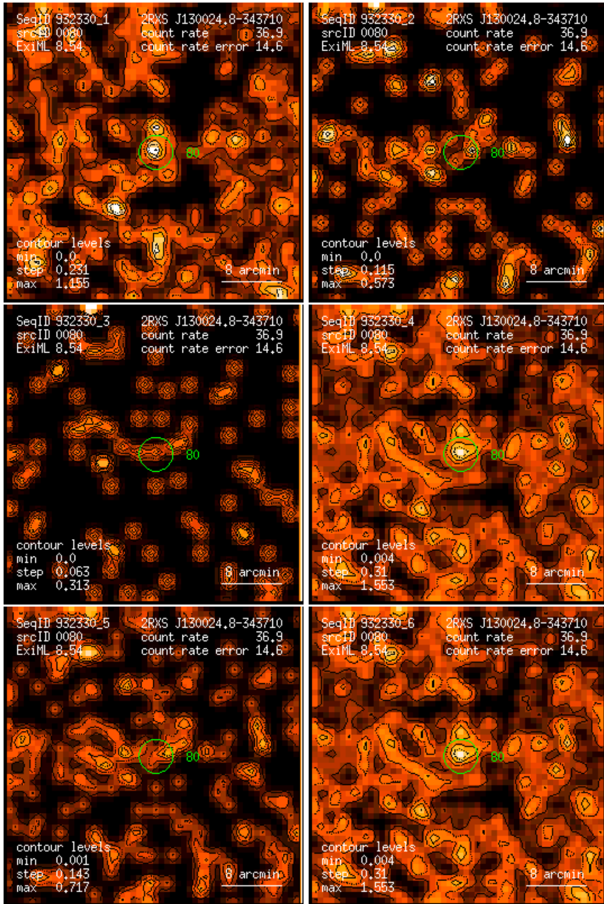
Figure 80: RASS 932330: detection 0080: band rate images, Gaussian filter: (1) PSPC channels 11 – 41, (2) 52 – 90, (3) 91 – 201, (4) 11 – 235, (5) 52 – 201, (6) 11 – 201. Broad band rates in counts/ks. Band rate contour levels in counts/ks/arcmin 2 .
