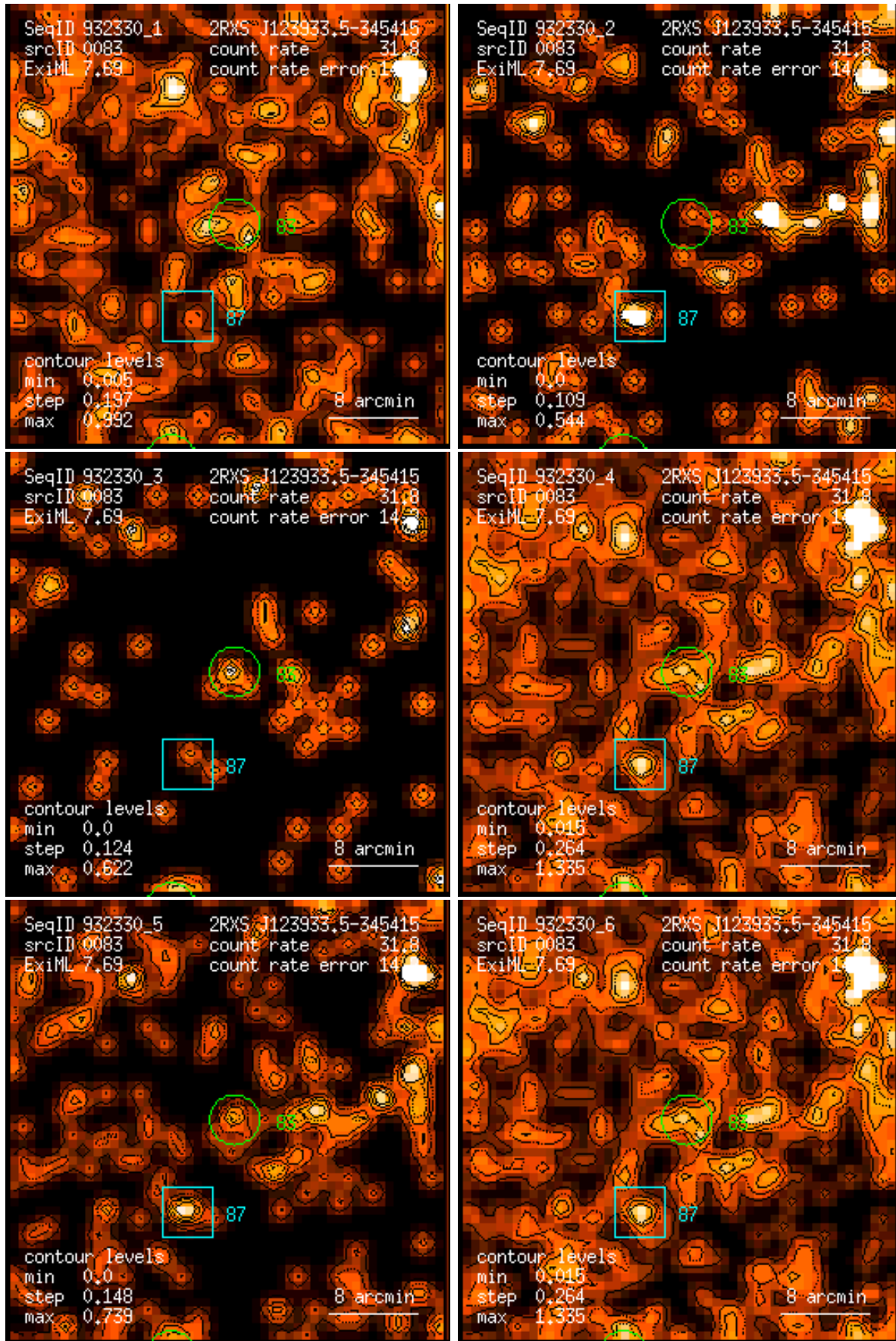
Figure 83: RASS 932330: detection 0083: band rate images, Gaussian filter: (1) PSPC channels 11 – 41, (2) 52 – 90, (3) 91 – 201, (4) 11 – 235, (5) 52 – 201, (6) 11 – 201. Broad band rates in counts/ks. Band rate contour levels in counts/ks/arcmin 2 .
