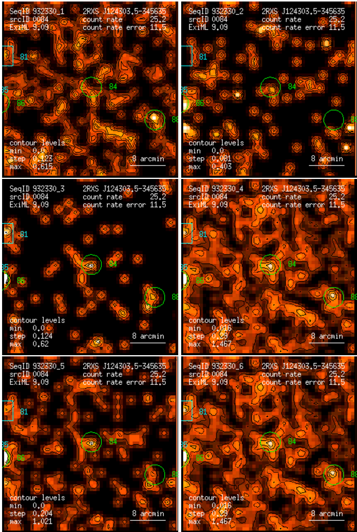
Figure 84: RASS 932330: detection 0084: band rate images, Gaussian filter: (1) PSPC channels 11 – 41, (2) 52 – 90, (3) 91 – 201, (4) 11 – 235, (5) 52 – 201, (6) 11 – 201. Broad band rates in counts/ks. Band rate contour levels in counts/ks/arcmin 2 .
