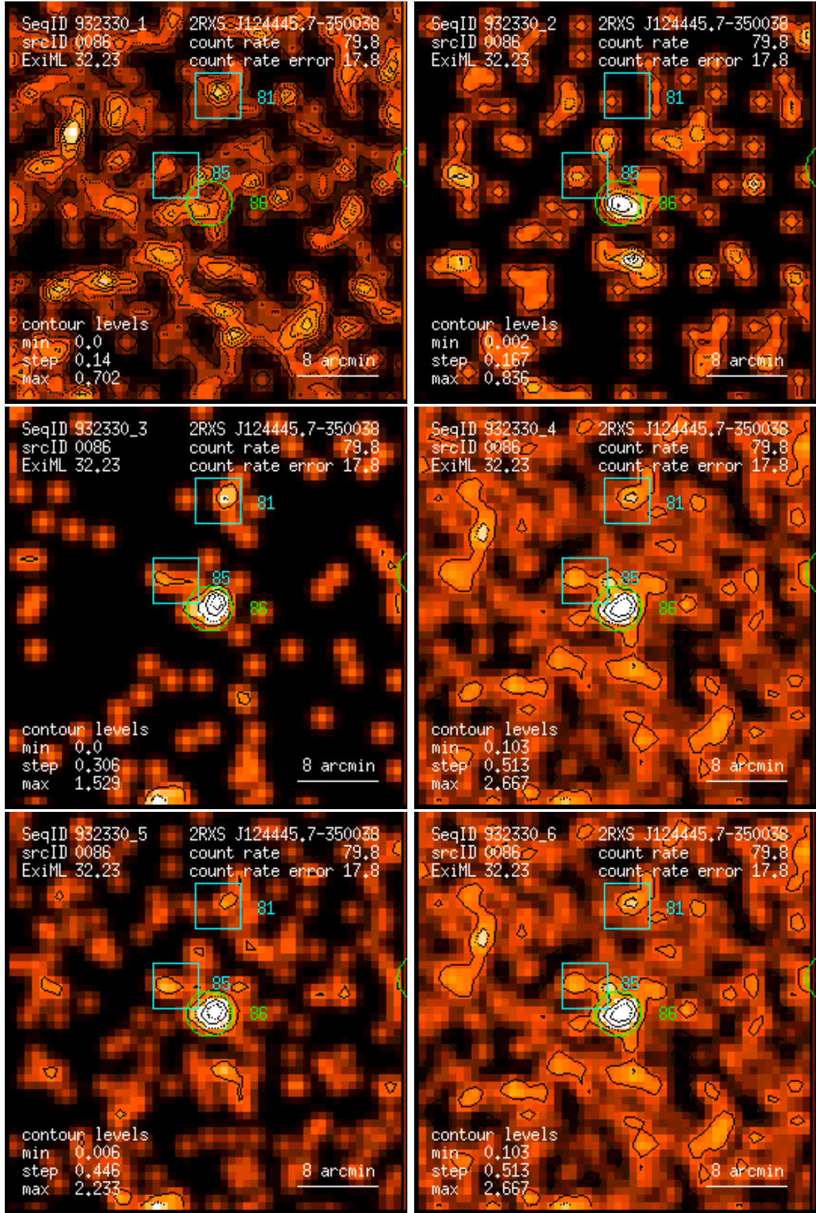
Figure 86: RASS 932330: detection 0086: band rate images, Gaussian filter: (1) PSPC channels 11 – 41, (2) 52 – 90, (3) 91 – 201, (4) 11 – 235, (5) 52 – 201, (6) 11 – 201. Broad band rates in counts/ks. Band rate contour levels in counts/ks/arcmin 2 .
