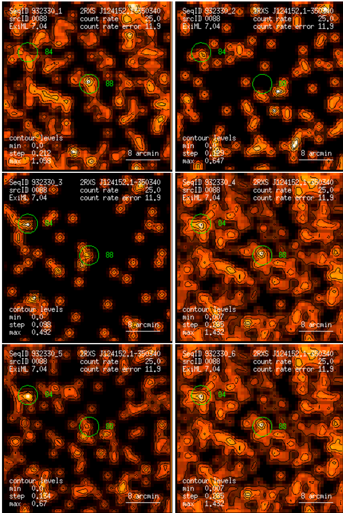
Figure 88: RASS 932330: detection 0088: band rate images, Gaussian filter: (1) PSPC channels 11 – 41, (2) 52 – 90, (3) 91 – 201, (4) 11 – 235, (5) 52 – 201, (6) 11 – 201. Broad band rates in counts/ks. Band rate contour levels in counts/ks/arcmin 2 .
