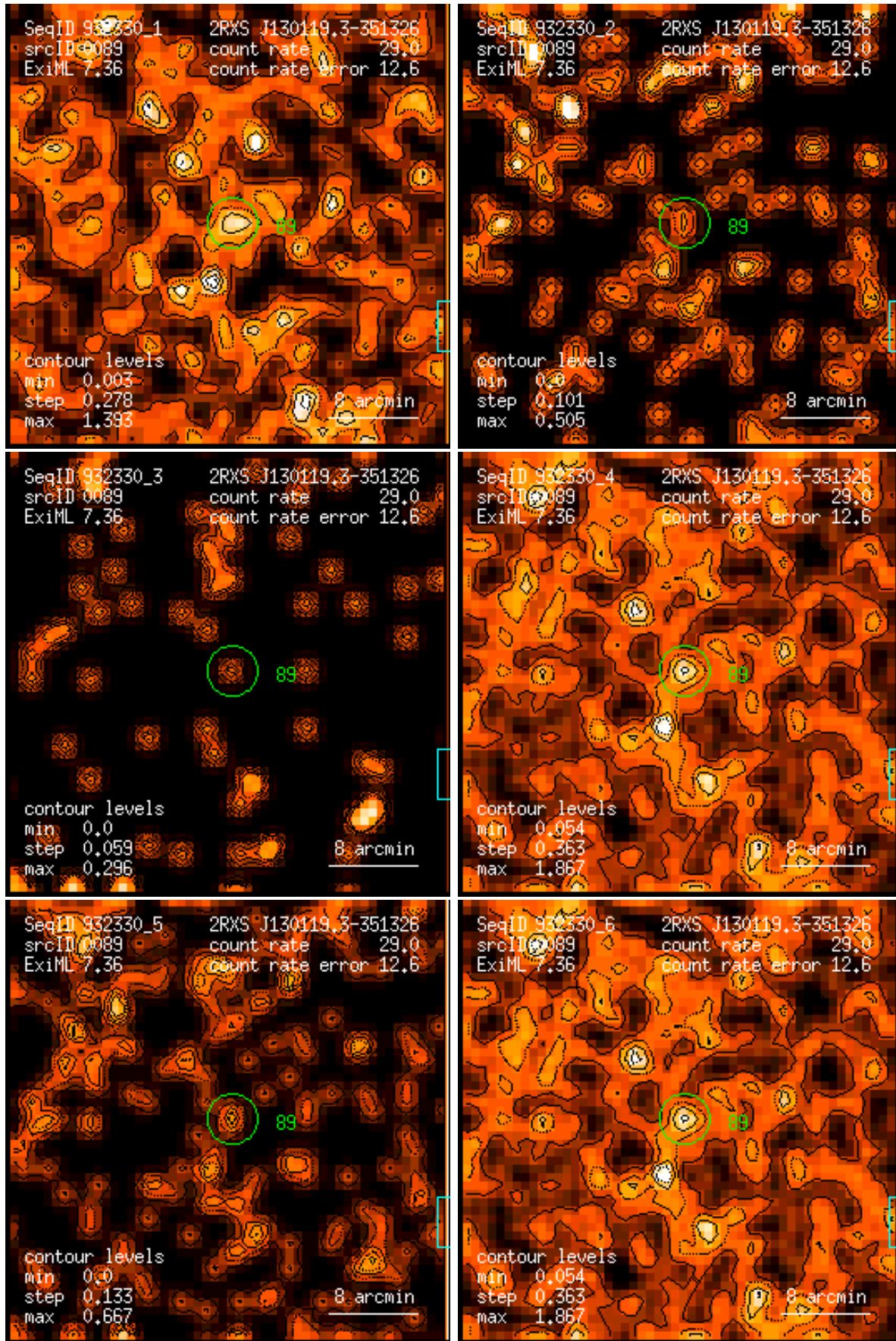
Figure 89: RASS 932330: detection 0089: band rate images, Gaussian filter: (1) PSPC channels 11 – 41, (2) 52 – 90, (3) 91 – 201, (4) 11 – 235, (5) 52 – 201, (6) 11 – 201. Broad band rates in counts/ks. Band rate contour levels in counts/ks/arcmin 2 .
