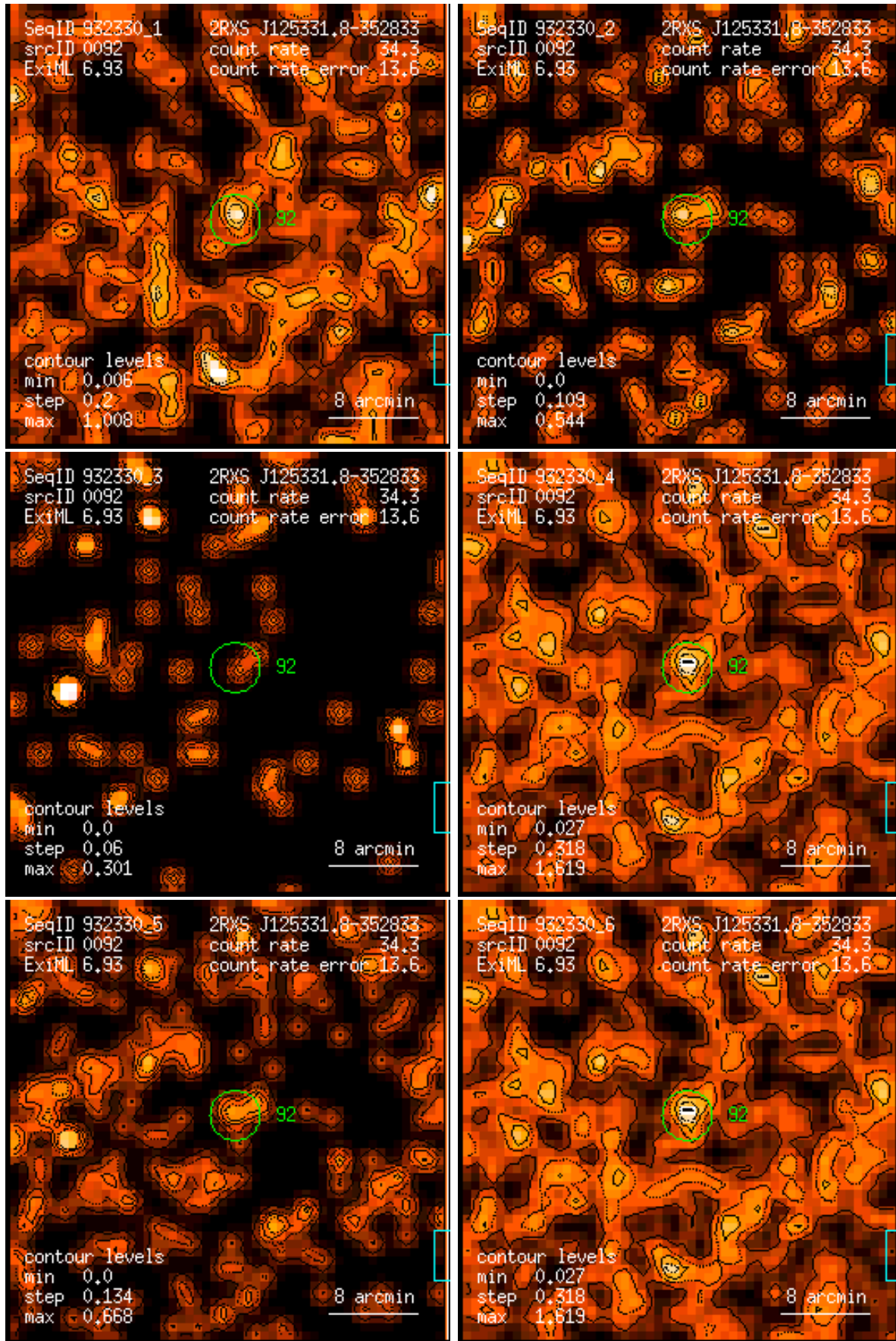
Figure 92: RASS 932330: detection 0092: band rate images, Gaussian filter: (1) PSPC channels 11 – 41, (2) 52 – 90, (3) 91 – 201, (4) 11 – 235, (5) 52 – 201, (6) 11 – 201. Broad band rates in counts/ks. Band rate contour levels in counts/ks/arcmin 2 .
