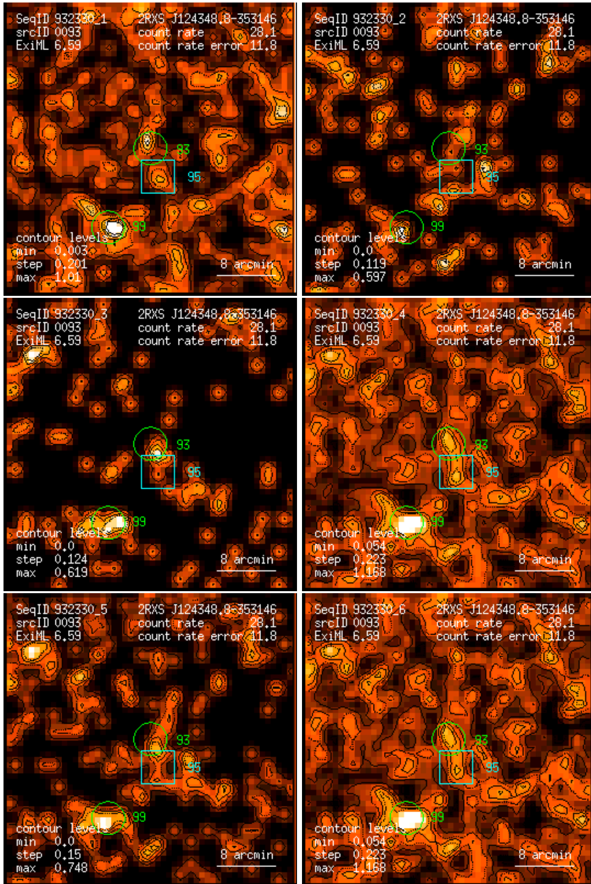
Figure 93: RASS 932330: detection 0093: band rate images, Gaussian filter: (1) PSPC channels 11 – 41, (2) 52 – 90, (3) 91 – 201, (4) 11 – 235, (5) 52 – 201, (6) 11 – 201. Broad band rates in counts/ks. Band rate contour levels in counts/ks/arcmin 2 .
