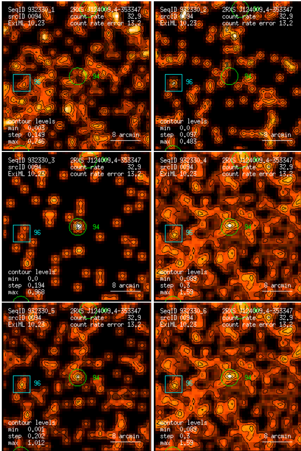
Figure 94: RASS 932330: detection 0094: band rate images, Gaussian filter: (1) PSPC channels 11 – 41, (2) 52 – 90, (3) 91 – 201, (4) 11 – 235, (5) 52 – 201, (6) 11 – 201. Broad band rates in counts/ks. Band rate contour levels in counts/ks/arcmin 2 .
