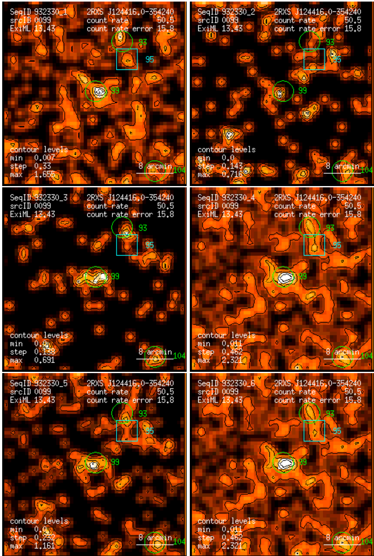
Figure 99: RASS 932330: detection 0099: band rate images, Gaussian filter: (1) PSPC channels 11 – 41, (2) 52 – 90, (3) 91 – 201, (4) 11 – 235, (5) 52 – 201, (6) 11 – 201. Broad band rates in counts/ks. Band rate contour levels in counts/ks/arcmin 2 .
