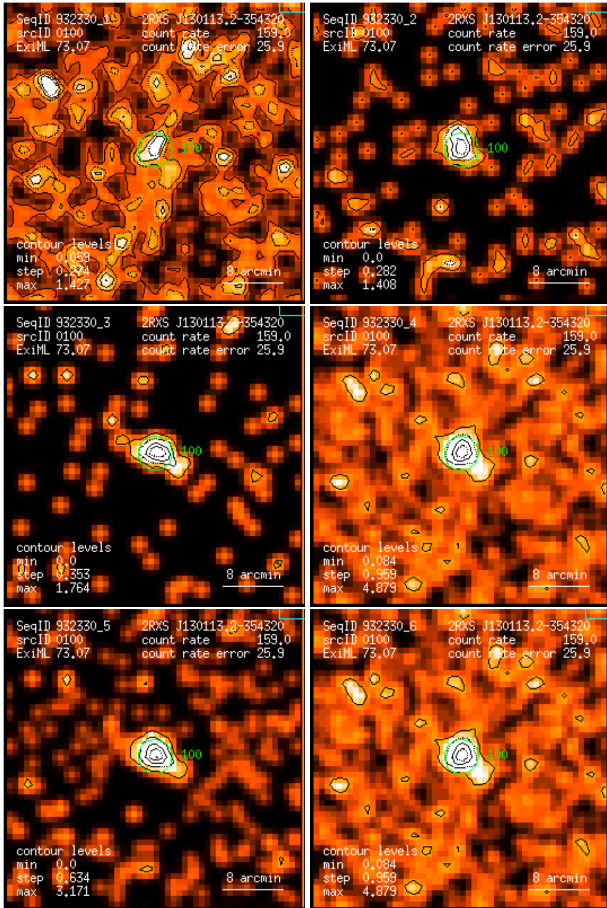
Figure 100: RASS 932330: detection 0100: band rate images, Gaussian filter: (1) PSPC channels 11 – 41, (2) 52 – 90, (3) 91 – 201, (4) 11 – 235, (5) 52 – 201, (6) 11 – 201. Broad band rates in counts/ks. Band rate contour levels in counts/ks/arcmin 2 .
