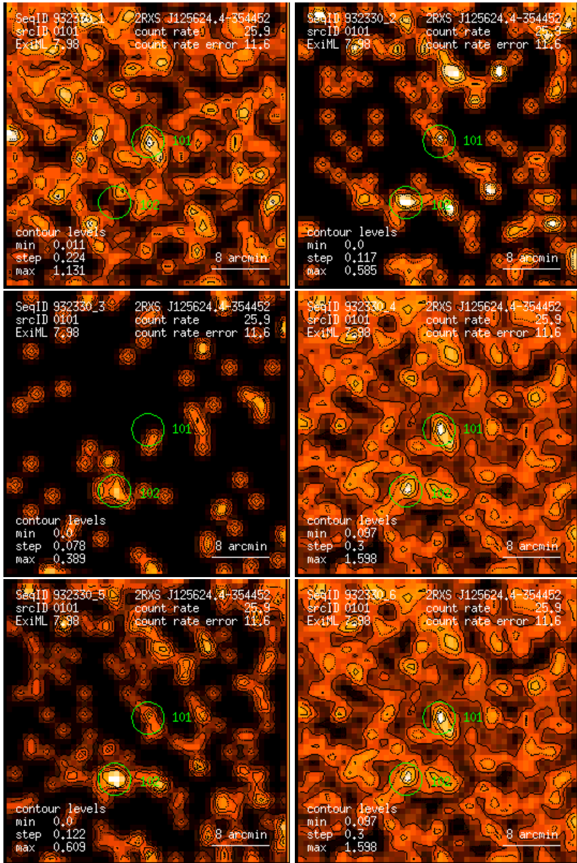
Figure 101: RASS 932330: detection 0101: band rate images, Gaussian filter: (1) PSPC channels 11 – 41, (2) 52 – 90, (3) 91 – 201, (4) 11 – 235, (5) 52 – 201, (6) 11 – 201. Broad band rates in counts/ks. Band rate contour levels in counts/ks/arcmin 2 .
