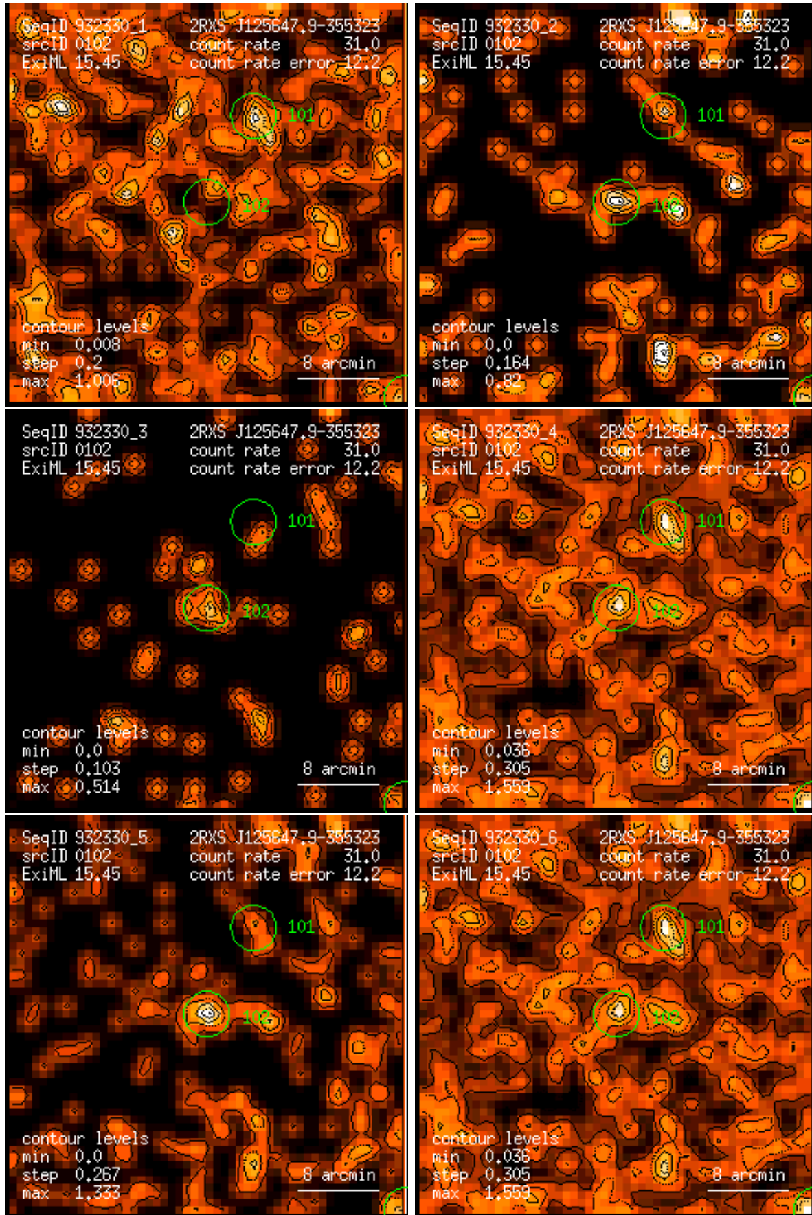
Figure 102: RASS 932330: detection 0102: band rate images, Gaussian filter: (1) PSPC channels 11 – 41, (2) 52 – 90, (3) 91 – 201, (4) 11 – 235, (5) 52 – 201, (6) 11 – 201. Broad band rates in counts/ks. Band rate contour levels in counts/ks/arcmin 2 .
