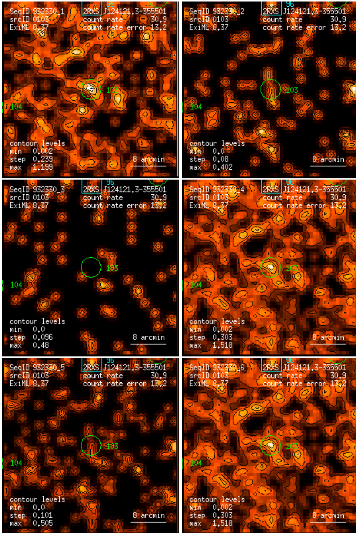
Figure 103: RASS 932330: detection 0103: band rate images, Gaussian filter: (1) PSPC channels 11 – 41, (2) 52 – 90, (3) 91 – 201, (4) 11 – 235, (5) 52 – 201, (6) 11 – 201. Broad band rates in counts/ks. Band rate contour levels in counts/ks/arcmin 2 .
