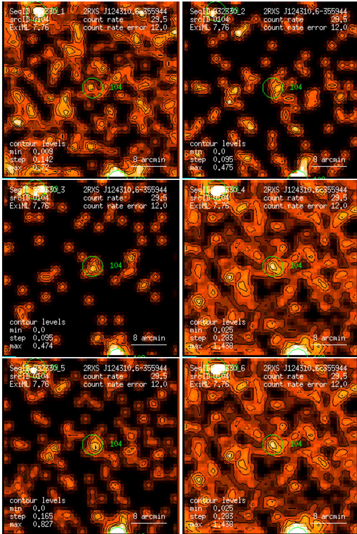
Figure 104: RASS 932330: detection 0104: band rate images, Gaussian filter: (1) PSPC channels 11 – 41, (2) 52 – 90, (3) 91 – 201, (4) 11 – 235, (5) 52 – 201, (6) 11 – 201. Broad band rates in counts/ks. Band rate contour levels in counts/ks/arcmin 2 .
