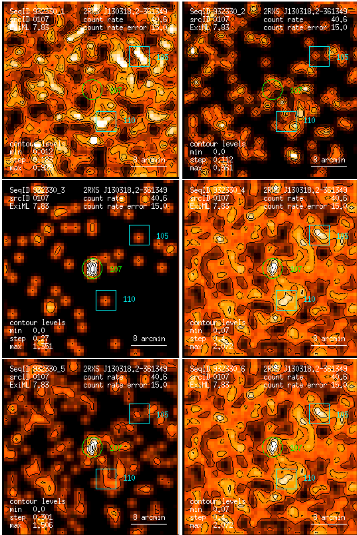
Figure 107: RASS 932330: detection 0107: band rate images, Gaussian filter: (1) PSPC channels 11 – 41, (2) 52 – 90, (3) 91 – 201, (4) 11 – 235, (5) 52 – 201, (6) 11 – 201. Broad band rates in counts/ks. Band rate contour levels in counts/ks/arcmin 2 .
