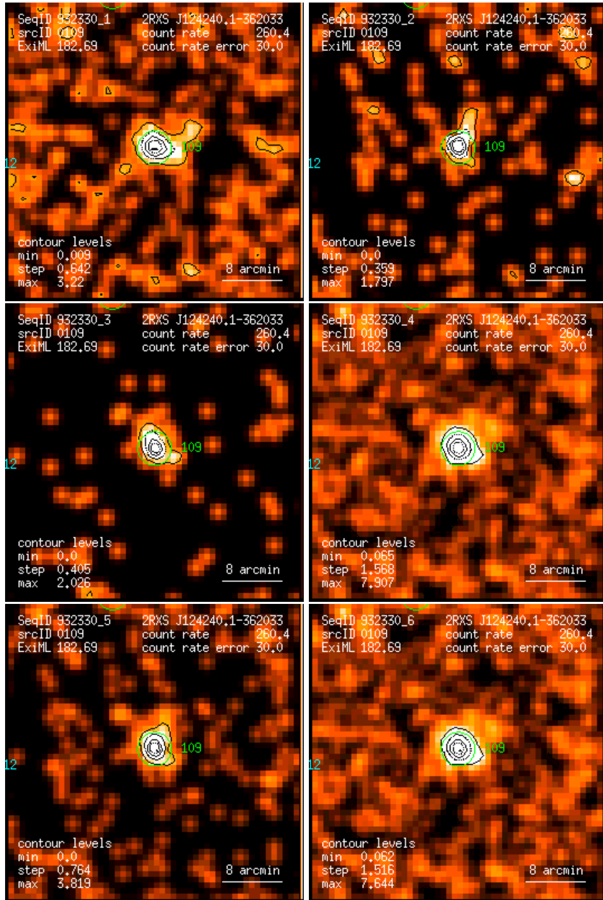
Figure 109: RASS 932330: detection 0109: band rate images, Gaussian filter: (1) PSPC channels 11 – 41, (2) 52 – 90, (3) 91 – 201, (4) 11 – 235, (5) 52 – 201, (6) 11 – 201. Broad band rates in counts/ks. Band rate contour levels in counts/ks/arcmin 2 .
