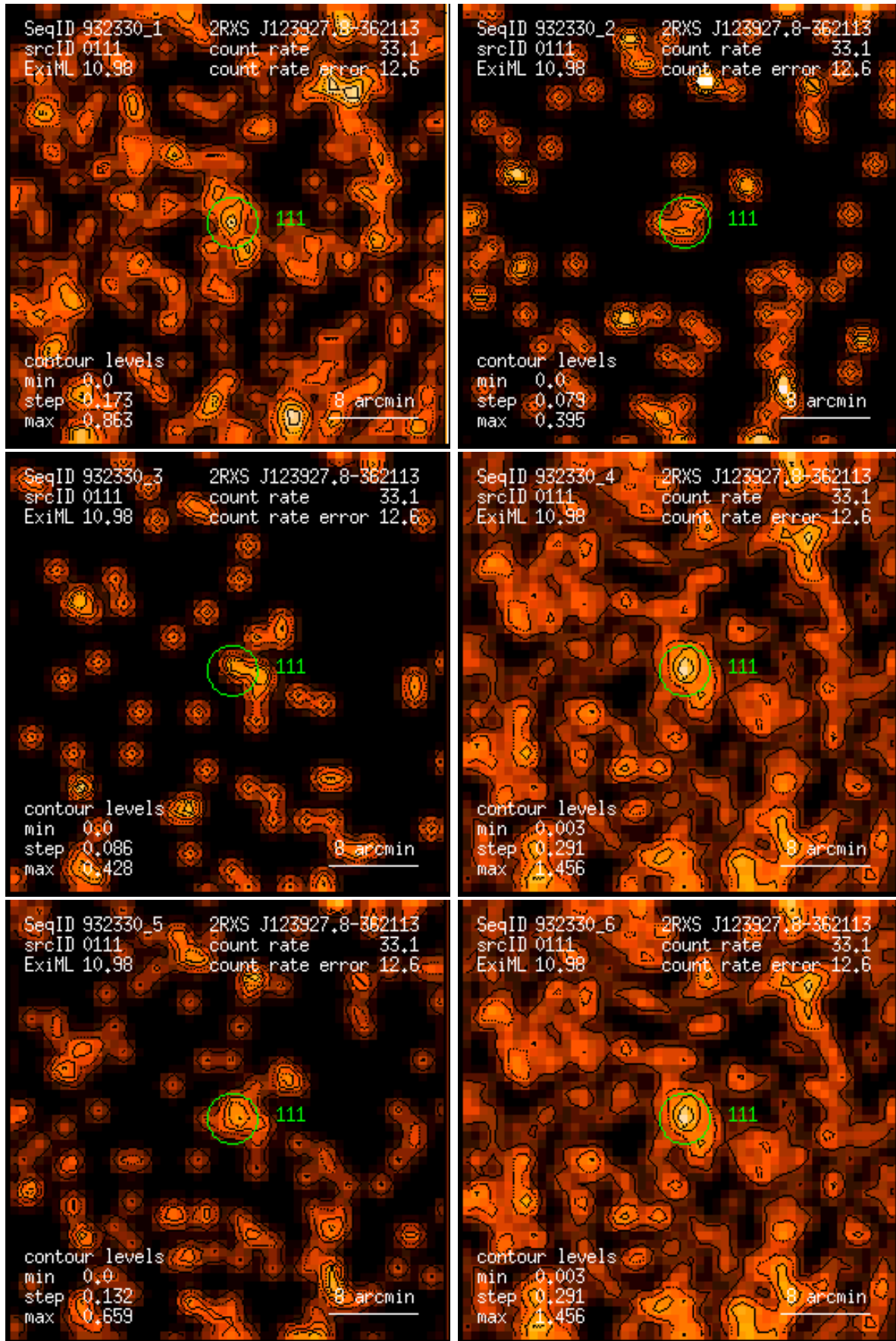
Figure 111: RASS 932330: detection 0111: band rate images, Gaussian filter: (1) PSPC channels 11 – 41, (2) 52 – 90, (3) 91 – 201, (4) 11 – 235, (5) 52 – 201, (6) 11 – 201. Broad band rates in counts/ks. Band rate contour levels in counts/ks/arcmin 2 .
