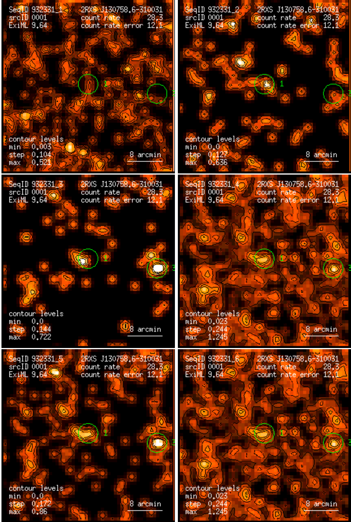
Figure 1: RASS 932331: detection 0001: band rate images, Gaussian filter: (1) PSPC channels 11 – 41, (2) 52 – 90, (3) 91 – 201, (4) 11 – 235, (5) 52 – 201, (6) 11 – 201. Broad band rates in counts/ks. Band rate contour levels in counts/ks/arcmin 2 .
