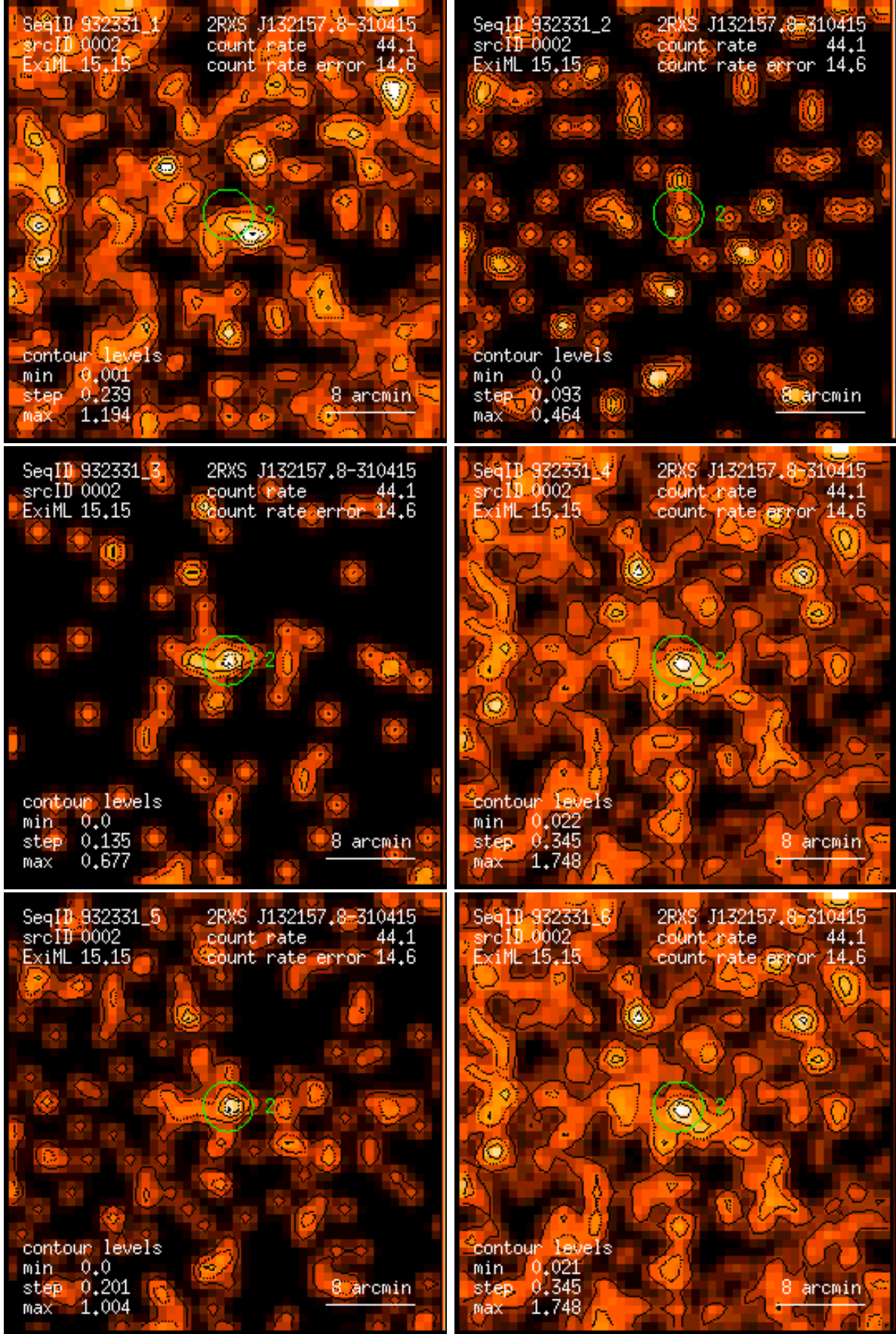
Figure 2: RASS 932331: detection 0002: band rate images, Gaussian filter: (1) PSPC channels 11 – 41, (2) 52 – 90, (3) 91 – 201, (4) 11 – 235, (5) 52 – 201, (6) 11 – 201. Broad band rates in counts/ks. Band rate contour levels in counts/ks/arcmin 2 .
