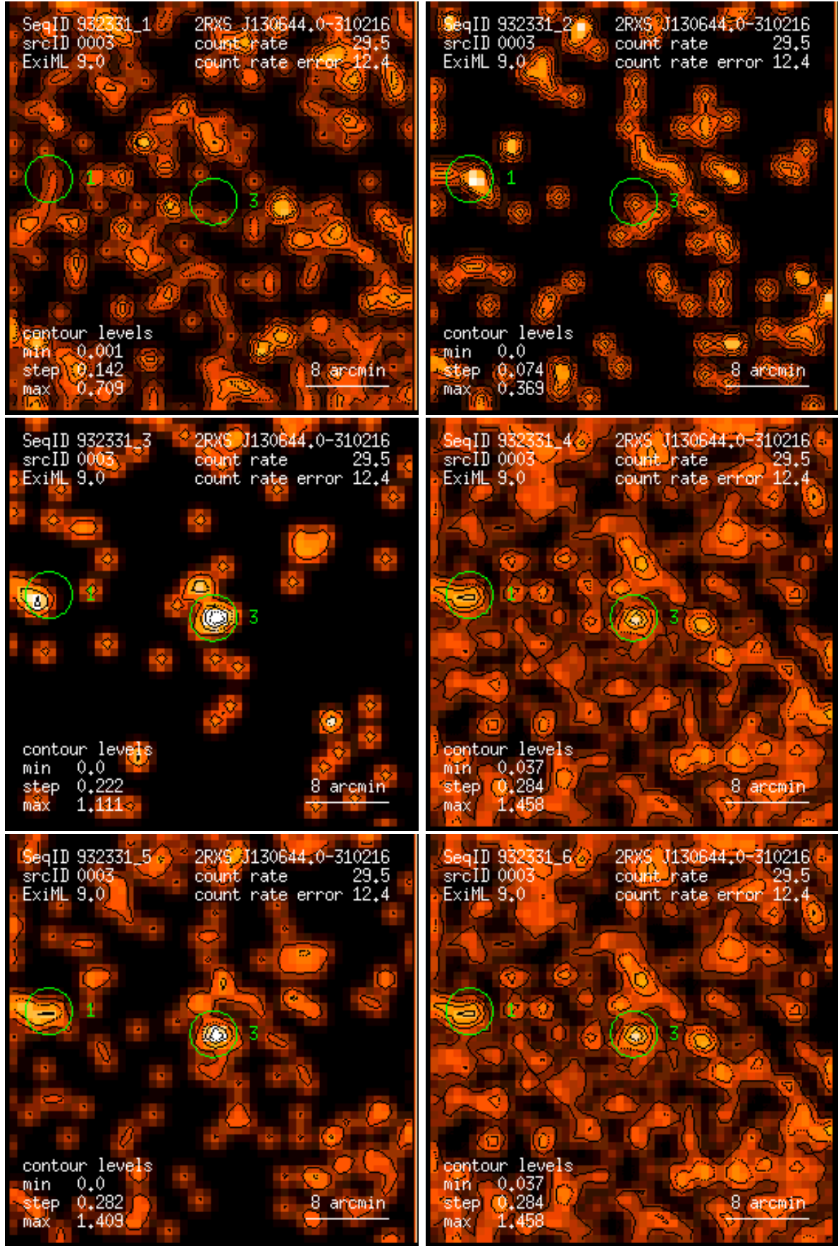
Figure 3: RASS 932331: detection 0003: band rate images, Gaussian filter: (1) PSPC channels 11 – 41, (2) 52 – 90, (3) 91 – 201, (4) 11 – 235, (5) 52 – 201, (6) 11 – 201. Broad band rates in counts/ks. Band rate contour levels in counts/ks/arcmin 2 .
