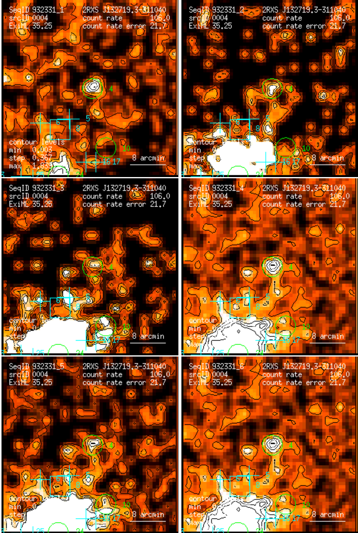
Figure 4: RASS 932331: detection 0004: band rate images, Gaussian filter: (1) PSPC channels 11 – 41, (2) 52 – 90, (3) 91 – 201, (4) 11 – 235, (5) 52 – 201, (6) 11 – 201. Broad band rates in counts/ks. Band rate contour levels in counts/ks/arcmin 2 .
