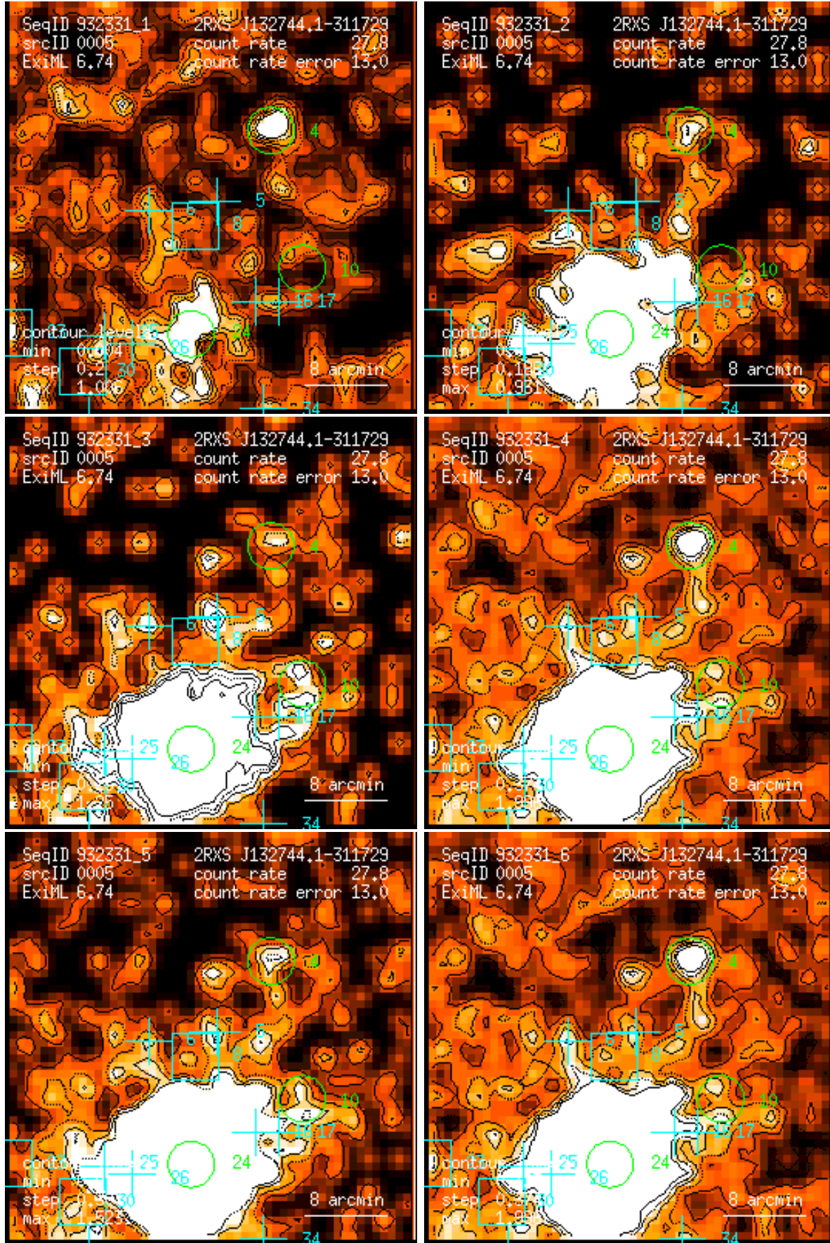
Figure 5: RASS 932331: detection 0005: band rate images, Gaussian filter: (1) PSPC channels 11 – 41, (2) 52 – 90, (3) 91 – 201, (4) 11 – 235, (5) 52 – 201, (6) 11 – 201. Broad band rates in counts/ks. Band rate contour levels in counts/ks/arcmin 2 .
