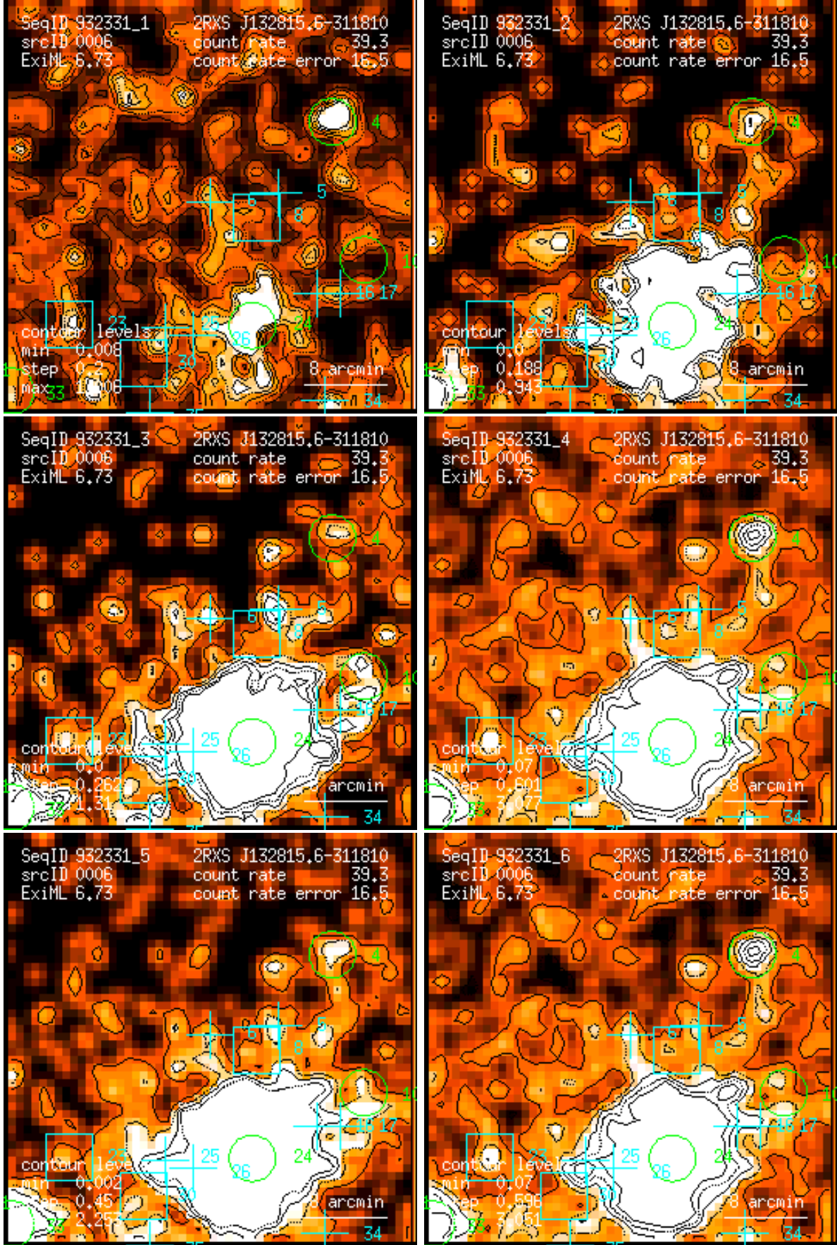
Figure 6: RASS 932331: detection 0006: band rate images, Gaussian filter: (1) PSPC channels 11 – 41, (2) 52 – 90, (3) 91 – 201, (4) 11 – 235, (5) 52 – 201, (6) 11 – 201. Broad band rates in counts/ks. Band rate contour levels in counts/ks/arcmin 2 .
