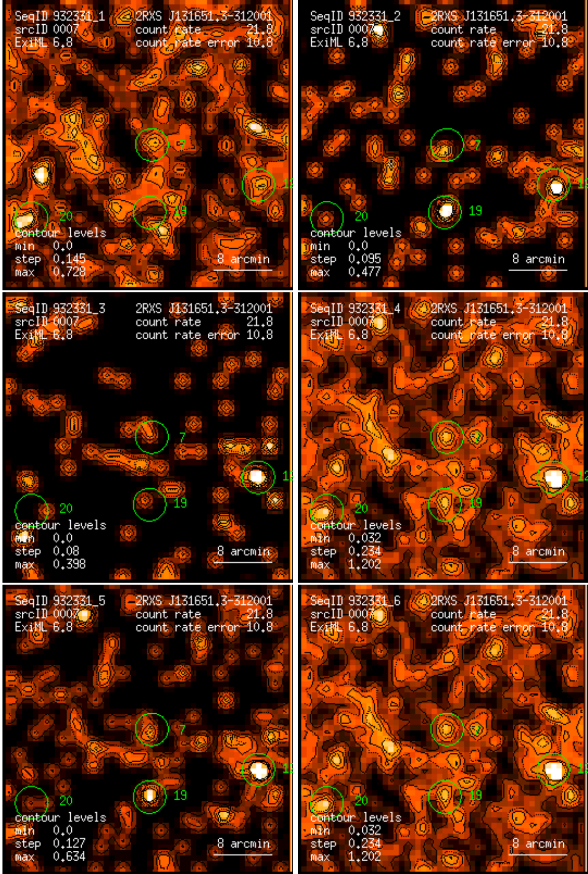
Figure 7: RASS 932331: detection 0007: band rate images, Gaussian filter: (1) PSPC channels 11 – 41, (2) 52 – 90, (3) 91 – 201, (4) 11 – 235, (5) 52 – 201, (6) 11 – 201. Broad band rates in counts/ks. Band rate contour levels in counts/ks/arcmin 2 .
